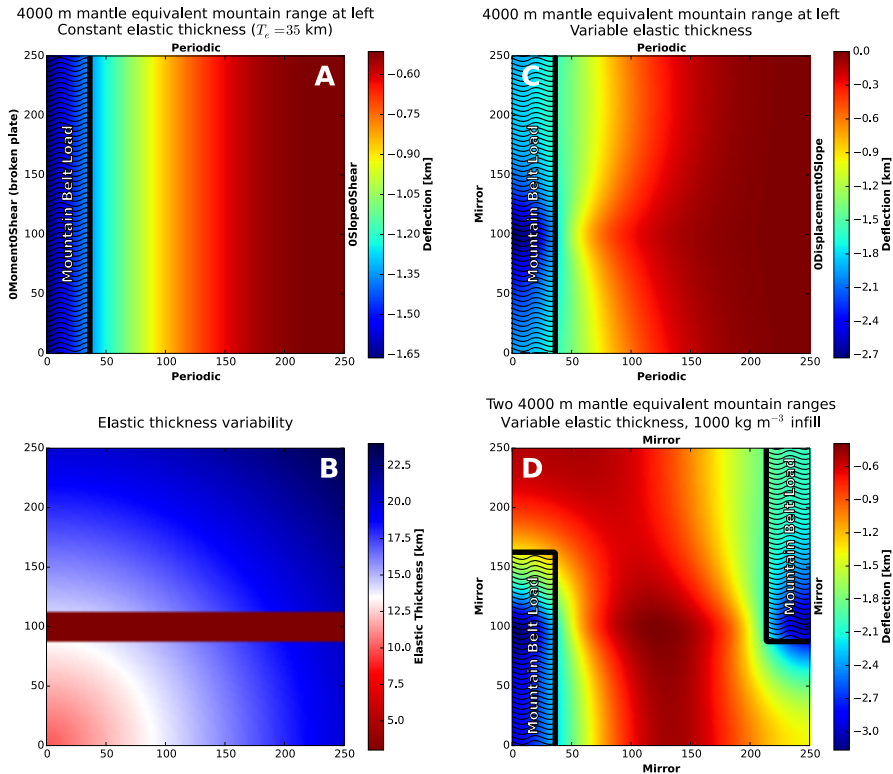
Figure 5. Example runs of gFlex with varying elastic thickness and boundary conditions. A depicts a long north–south mountain belt and foreland basin under uniform elastic thickness. B provides a contrived field of variable elastic thickness. C is similar to A except in that it uses a mirror boundary for a symmetrical mountain belt over a continuous lithospheric plate instead of a broken plate solution, and that the plate has the variable elastic thickness structure given in B . D depicts the flexural interaction of two mountain belts on the same variable-elastic-thickness lithosphere shown in B and has mirror boundary conditions at all edges.
