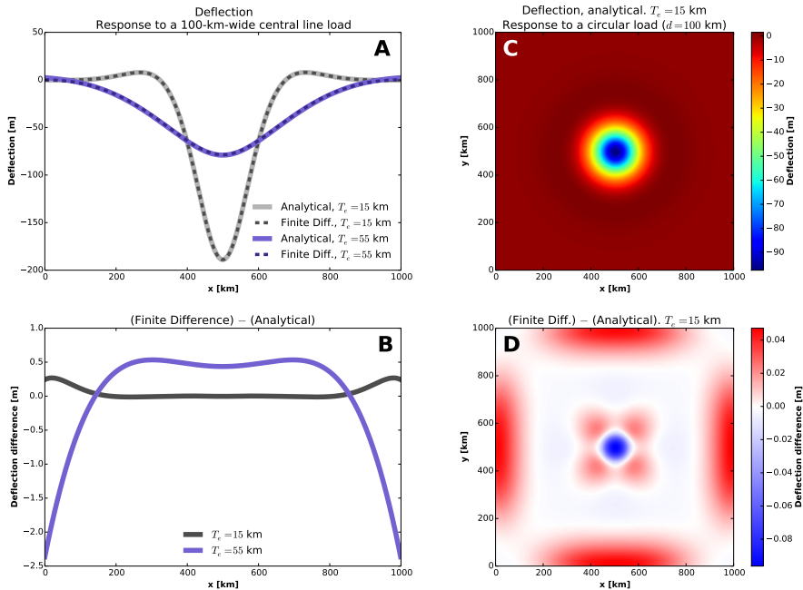
Figure 3. Numerical (FD) and analytical (SAS) solutions in 1D (A) and 2D (C) and their differences (B and D) in response to a 100-km-(long/in-diameter) central line/circular load. These differences are due primarily to the NoOutsideLoads boundary condition of the analytical solution and the 0Displacement0Slope boundary condition of the numerical solution. This can be seen in panel B where the example with a lower elastic thickness is less-offset due to the greater number of flexural wavelengths between the load and the boundary, and in the greater agreement between the solutions on the longer diagonal boundaries in D. The offset in the middle, visible as a small bump in B and a blue diamond surrounded by red petals in D, is due to the difference between approximating the load as a sum of point impulses (analytical) and as the solution to a rectangularly gridded matrix equation based on the same theory (numerical).
