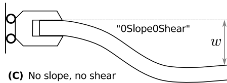
(C) No slope, no shear (plate boundary clamped but free to translate up and down)
