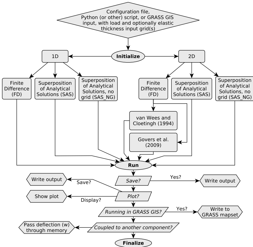
Figure 2. Flowchart for gFlex as (1) a standalone model with configuration and input files, (2) a Python module or coupled component in a modeling framework, or (3) a GRASS GIS component.
