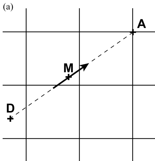
Figure 1. Schematic of two-dimensional advection for (a) the traditional backward semi-Lagrangian scheme and (b) the NDSL scheme. “D,” “M,” and “A” indicate the departure point, mid-point, and arrival point, respectively. The bold arrow indicates the wind vector at the mid-point.
