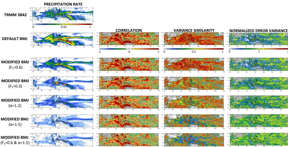
Figure 3. Precipitation rate ( \text{mm h}^{-1} ) from TRMM and WRF and model correlation ( \rho ), variance similarity ( \eta ) and normalized error variance ( \alpha_e ) with respect to TRMM for the experiments with the default BMJ scheme and with five modified versions of the BMJ scheme averaged over April 2008. The conventions are as in Fig. 1 with regions where \rho , \eta and \alpha_e are infinite shaded in grey.
