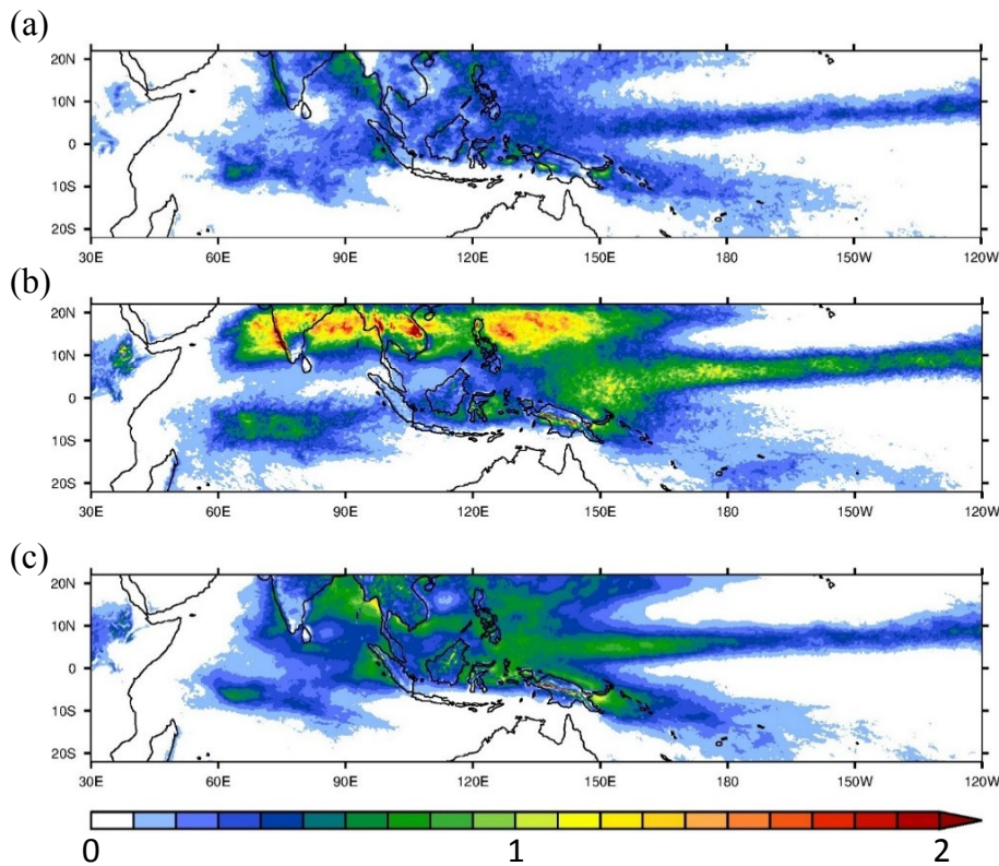
Figure 1. Precipitation rate (units of \text{mm h}^{-1} ) averaged over June to September (JJAS) 2008 from (a) TRMM 3B42 version 6, (b) WRF run with no interior nudging and (c) WRF run with analysis nudging (see text for more details). In all plots the colour bar is linear with only the middle and end values shown.
