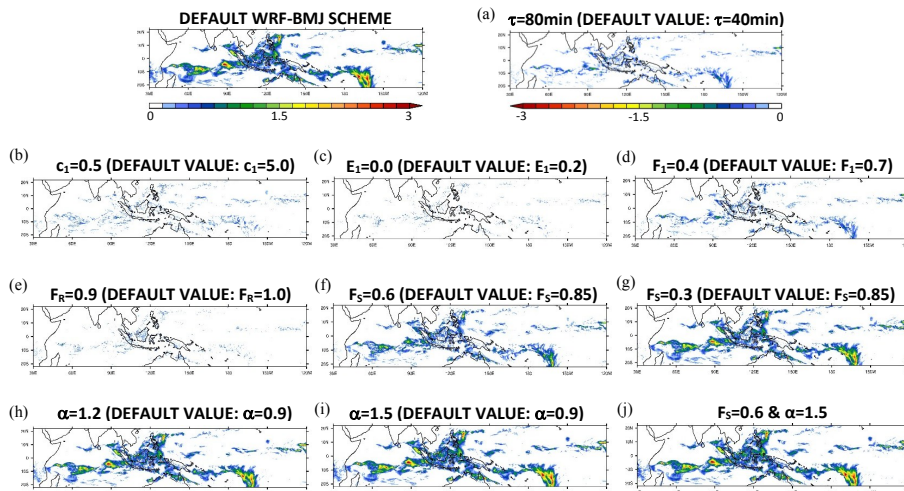
Figure 2. Precipitation rate from a 1 day WRF run (from 00:00 UTC on 2 March to 00:00 UTC on 3 March 2008) with the default WRF-BMJ and modification in the rainfall rate for ten experiments with a modified BMJ scheme using separately (a) \tau = 80 min, (b) c_1 = 0.5 , (c) E_1 = 0.0 , (d) F_1 = 0.4 , (e) F_R = 0.9 , (f) F_S = 0.6 , (g) F_S = 0.3 , (h) \alpha = 1.2 , (i) \alpha = 1.5 and (j) F_S = 0.6 and \alpha = 1.5 (units of \text{mm h}^{-1} ). The conventions are as in Fig. 1. Note that the colour scale is reversed to show drying upon modifications.
