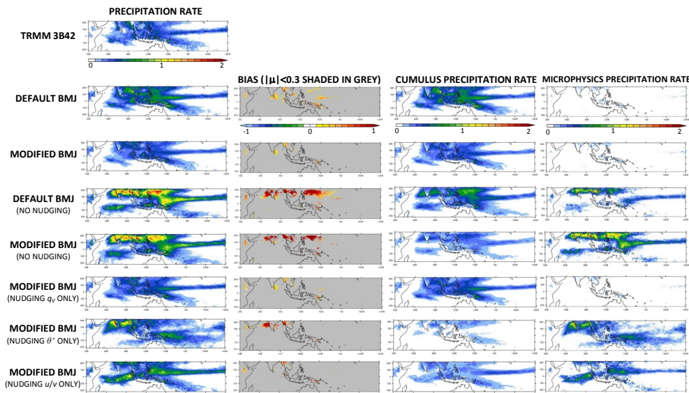
Figure 4. Precipitation rate ( \text{mm h}^{-1} ) averaged over JJAS 2008 from TRMM and 7 WRF experiments with the default BMJ and modified BMJ ( F_S = 0.6 ) schemes both with and without analysis nudging and relaxing only the water vapour mixing ratio ( q_v ), horizontal winds ( u , v ) and potential temperature perturbation ( \theta' ) in the interior of the domain separately towards CFSR. Left to right: precipitation rate, model bias (regions where |\mu| < 0.3 are shaded in grey) with respect to TRMM and precipitation rate from the cumulus and microphysics schemes. The conventions are as in Fig. 1.
