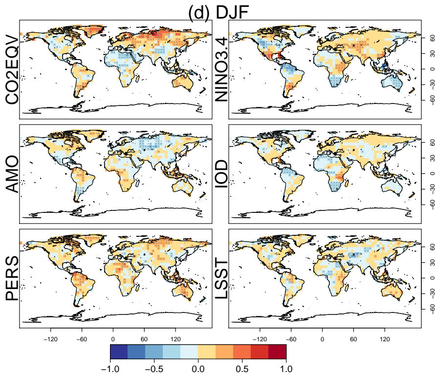
Figure 2. Correlation between PREC and the set of predictors (1961–2013) for (a) MAM, (b) JJA, (c) SON and (d) DJF. As in Figure 1, correlation between CO2EQV is shown in the top left panel; subsequent panels show correlation between predictand–predictor pairs following removal of the CO2EQV trend. Stippling is used to indicate significance at the 95% level.
