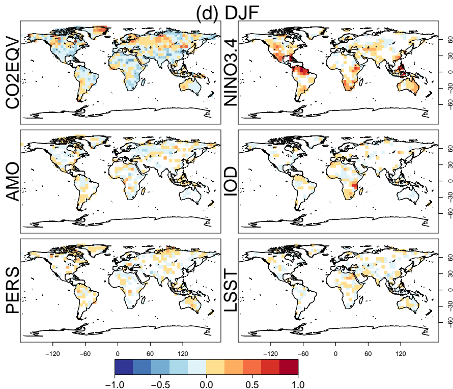
Figure 6. Correlation between PREC hindcasts and observations (1961–2013) for (a) MAM; (b) JJA, (c) SON and (d) DJF. The top left panel shows correlation between observations and SAT hindcasts constructed using CO 2 -equivalent as the sole predictor; stippling is used to indicate significance at the 95% level. Subsequent panels show difference in correlation following the inclusion of additional predictors.
