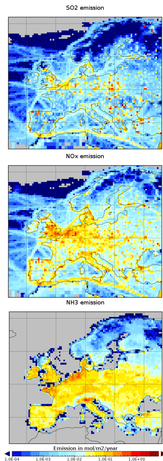
Figure 9. Maps of annual emissions for sulfur dioxide (top panel), nitrous oxides (middle panel) and ammonia (bottom panel) in \text{mol m}^{-2} \text{ year}^{-1} for the MOCAGE simulations (RACM and RACMSIA).
