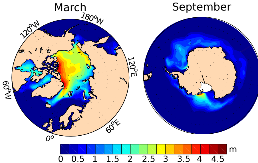
Figure 5. Mean simulated sea ice thicknesses (in m) at the time of the maximum ice volume: for March in the Northern Hemisphere and for September in the Southern Hemisphere.
