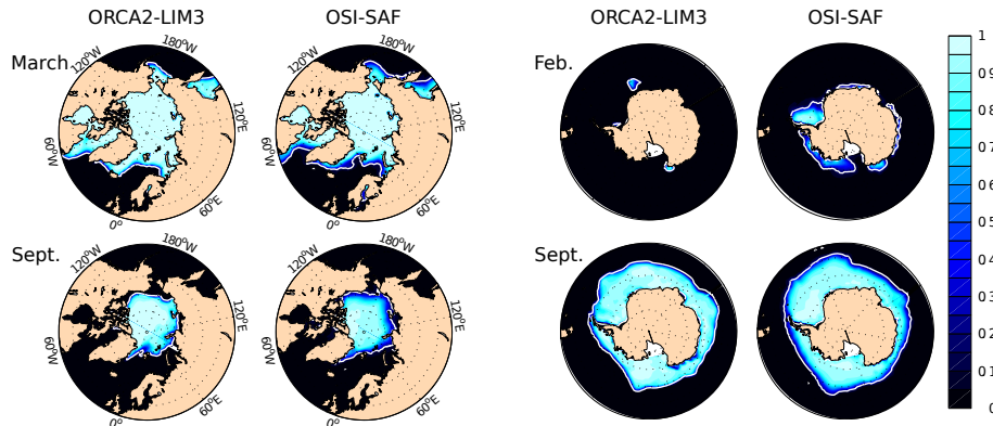
Figure 3. Mean sea ice concentrations from the simulation ORCA2-LIM3 and the observations OSI-SAF for March and September in the Arctic (left panels) and February and September in the Antarctic (right panels). The white line delimits the 15% ice concentration contour.
