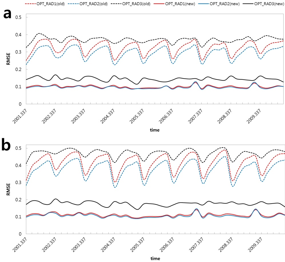
Figure 7. Comparison of RMSE values of albedo with the original minimum value of LAI and SAI (dashed lines) vs. new LI and SI (solid lines) for three radiation options for (a) BATS and (b) CLASS radiation schemes. OPT_RAD1 is MTSA, OPT_RAD2 is two-stream radiation option with no canopy gap, and OPT_RAD3 is the scheme that calculate the gap from vegetation fraction.
