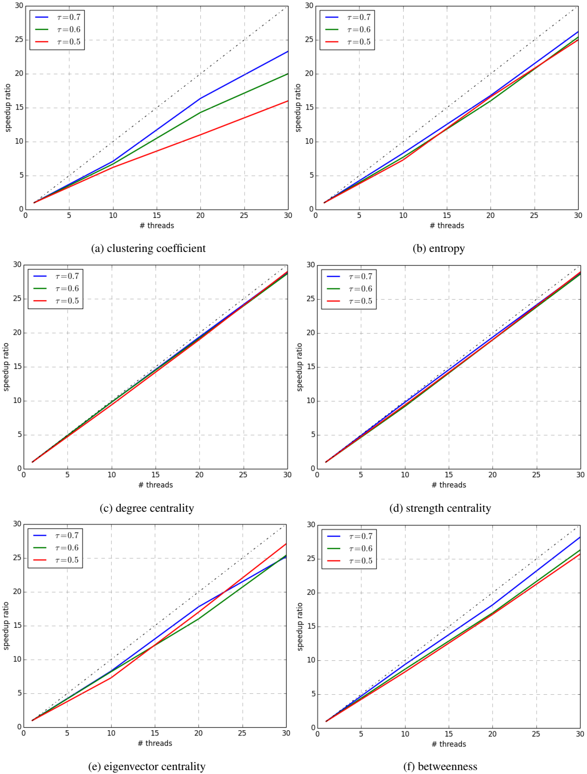
Fig. 5: Performance of the parallel algorithms running on a single SMP bullx node of 30 compute cores. The speedup ratios correspond to the analysis of the networks 1-3 presented in Table 1.
