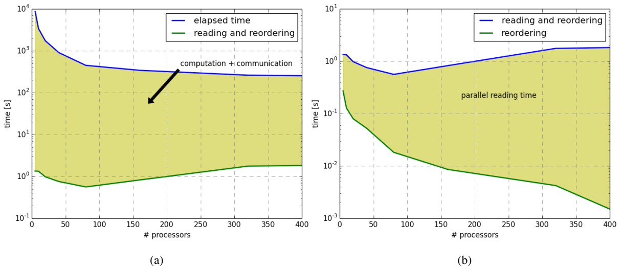
Fig. 4: In (a) the overall runtime of the experiment in Fig. 3b (for \tau = 0.5 ) is shown in the upper curve and compared to the time for parallel reading and reordering of time series (the lower curve). The shaded area corresponds to real cpu time for the calculation of the correlation matrix and the communication between processors. Both times for parallel reading and reordering preprocessing tasks are shown respectively in (b).
