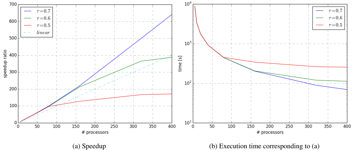
Fig. 3: Speedup ratio (a) for the parallel construction of SSH climate networks from the POP model data having 0.4^\circ spatial resolution. The shown speedup also includes the parallel reading and reordering of the input time series. The corresponding execution times (in seconds) over different sizes of computing processors starting from 5 processors upwards is given in (b).
