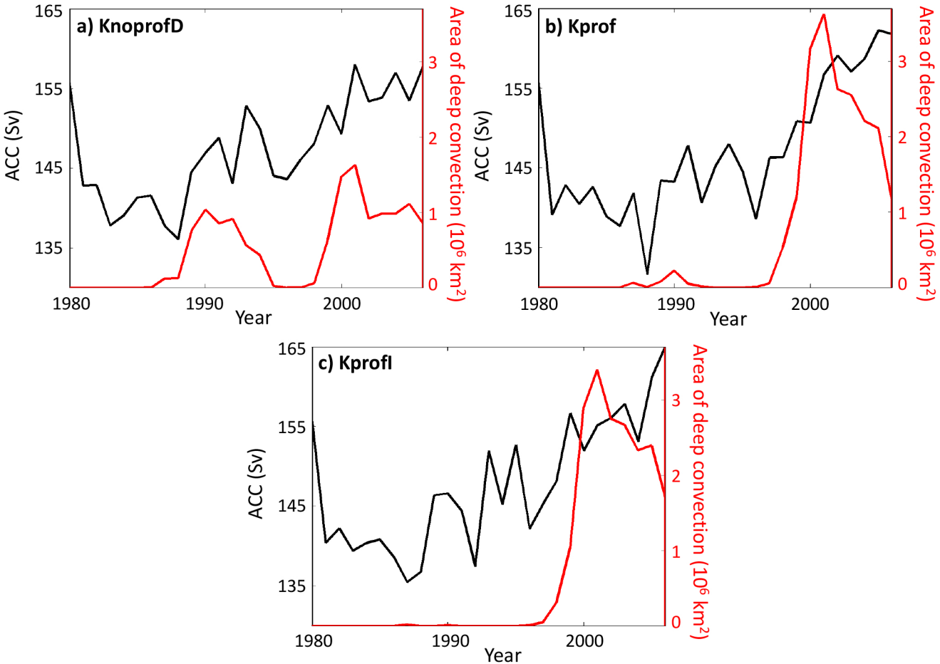
27-year time series of the annual maximum ACC (black) and annual maximum area of deep convection in the Southern Ocean (red).
