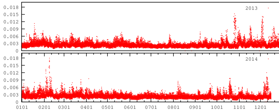
Figure 16. Time series of the maximum value of the amplitude in the mean sea level pressure variations (Eq. 3) computed from the coupling files from ARPEGE.
