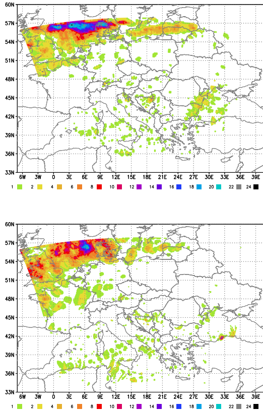
Figure 10. Spatial distribution of the number of occurrences when IFSM (top) and MCUF (bottom) values exceed the value 0.003, for forecast hour greater than or equal to 6 h for the period since 1 November 2010 until 15 November 2014.
