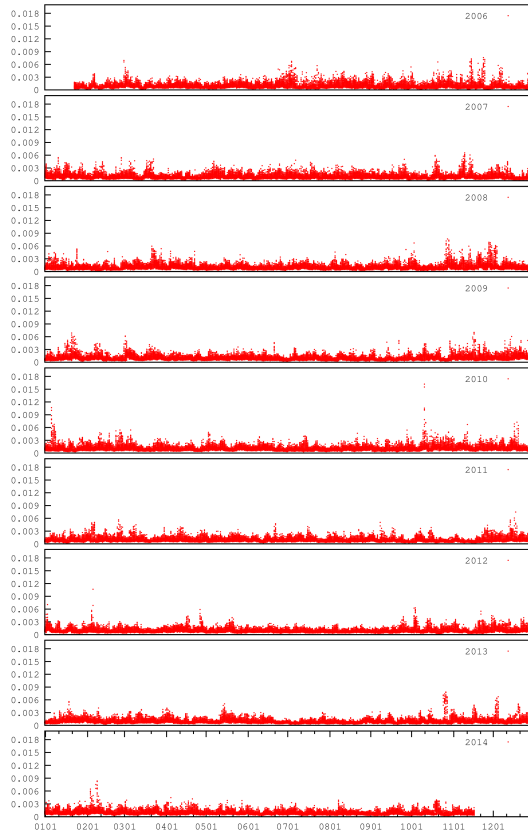
Figure 3. Maximum value of the MCF field (units 0.001 hPa) on the LACE coupling domain, provided from ARPEGE, from the coupling files for 6 h forecast up to 72 h forecast (60 h for 18:00 UTC run), starting from 00:00, 06:00, 12:00 and 18:00 UTC analyses, since 23 January 2006 until 15 November 2014.
