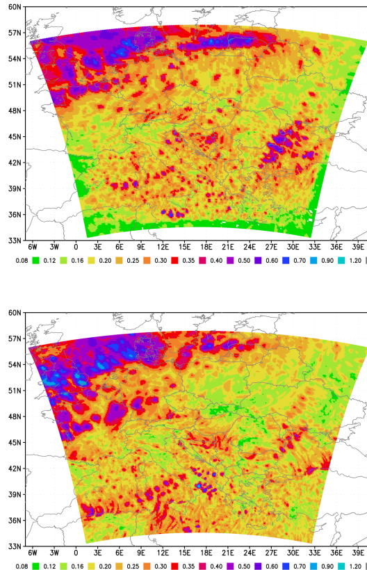
Figure 9. Spatial distribution of the maximum of absolute IFSM (top) and MCUF (bottom) (units 0.001 hPa), for forecast hour greater than or equal to 06 h for the period since 1 November 2010 until 15 November 2014.
