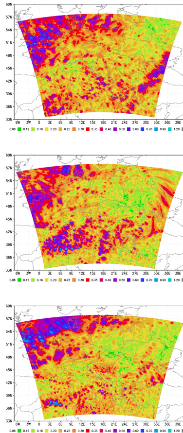
Figure 6. Absolute maximum values of the MCF field (units 0.001 hPa) from ARPEGE for different resolutions of the coupling files: (a) 20.678 km averaged for the period 23 January 2006 to 6 February 2008. (b) 15.4 km averaged for the period 6 February 2008 to 11 May 2010. (c) 10.51 km averaged for the period 11 May 2010 to 15 November 2014.
