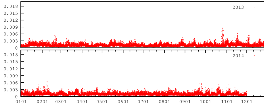
Figure 11. Time series of maximum value of ARPM (MCUF computed by running ALADIN on the coupling LACE domain from ARPEGE (the domain and resolution of LBC files) with 450 s time-step).
