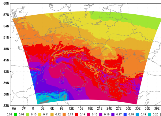
Figure 8. Spatial distribution of the average IFSM (top) and MCUF (bottom) values (units 0.001 hPa) for forecast hour greater than or equal to 06 h for the period since 1 November 2010 until 15 November 2014.
