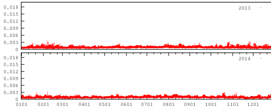
Figure 13. Time series of maximum value of error function, fields are initialized with DFI.
