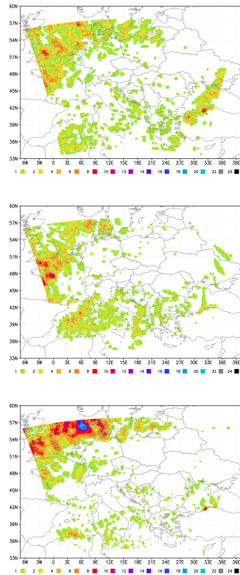
Figure 5. The number of times the MCUF field from ARPEGE exceeds 0.003 threshold for different resolutions of the coupling files: (a) 20.678 km averaged for the period 23 January 2006 to 6 February 2008. (b) 15.4 km averaged for the period 6 February 2008 to 11 May 2010. (c) 10.51 km averaged for the period 11 May 2010 to 15 November 2014.
