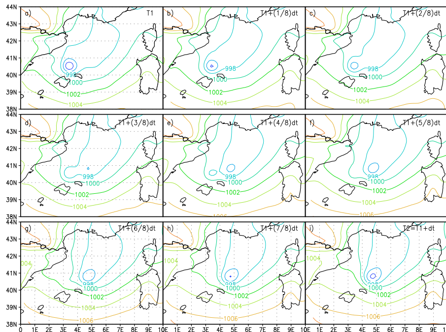
Figure 2. Mean sea level pressure (hPa) from ARPEGE operational coupling files starting from 12:00 UTC analysis on 27 October 2008, 57 (a) and 60 (i) hour forecasts, linear interpolation of mslp in time to half of the 3h coupling period (e), 1/8 of 3h (b), 1/4 (c) 3/8 (d), 5/8 (f), 3/4 (g) and 7/8 (h).
