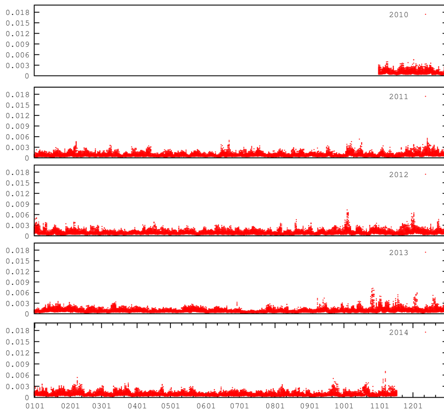
Figure 7. Time series of maximum value of IFSM field (units 0.001 hPa) on the coupling LACE domain for 6 h forecast up to 78 h forecast, computed by running ALADIN, starting from 00:00, 06:00, 12:00 and 18:00 UTC analyses, since 1 November 2010 until 15 November 2014.
