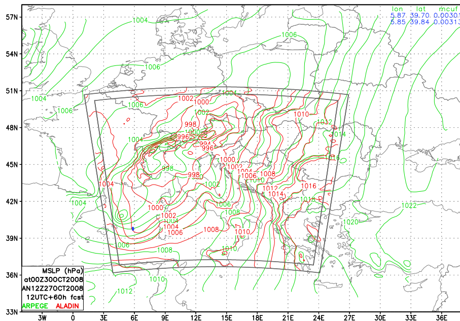
Figure 1. Mean sea level pressure (hPa) from ARPEGE (green) and ALADIN (red) operational 60 h forecast starting from 12:00 UTC analysis on 27 October 2008. The coordinates and values of MCUF field exceeding the 0.003 threshold are listed in the upper right corner and plotted as blue dots on the map.
