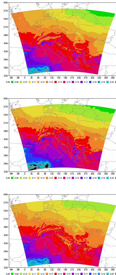
Figure 4. Average MCUF field (units 0.001 hPa) from ARPEGE for different resolutions of the LACE coupling files: (a) 20.678 km averaged for the period 23 January 2006 to 6 February 2008. (b) 15.4 km averaged for the period 6 February 2008 to 11 May 2010. (c) 10.51 km averaged for the period 11 May 2010 to 15 November 2014.
