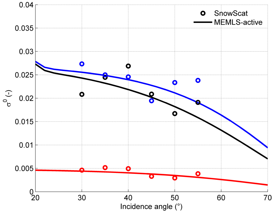
Figure 9. \sigma^0 at 10.2 GHz measured by SnowScat (circles) and modeled by MEMLS3&a with CT input (lines). Colors represent polarization, with vv – black, hh – blue and hv – red. Best fit parameters according to Fig. 8.
