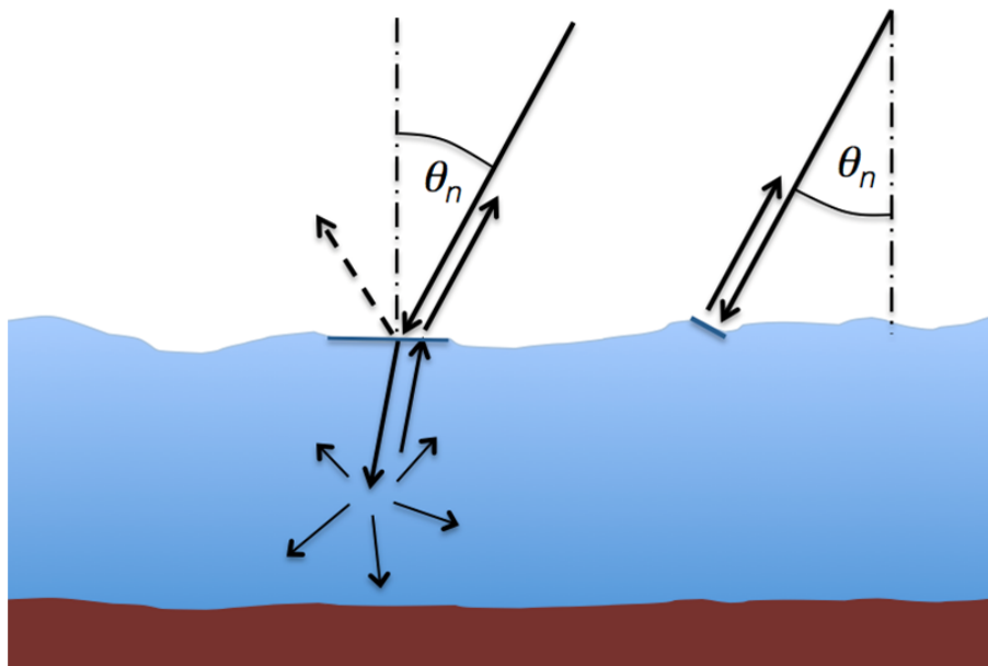
Figure 1. Snowpack (blue) with slightly undulated snow surface and layers. Waves incident at nadir angle \theta_n are refracted at the snow surface followed by volume scattering with backscatter; specular reflection without backscatter (left). Specular backscatter from a slightly tilted patch of the surface (right) and layer interfaces (not shown).
