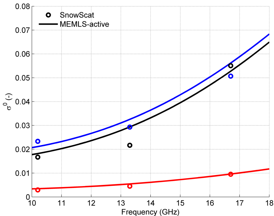
Figure 8. \sigma_0^0 at incidence angle 50^\circ measured by SnowScat (circles) and modeled by MEMLS3&a with CT input (lines) for best fit parameters s_{s0,h} = 0.75 \cdot s_{0,h} , s_{s0,v} = 0.75 \cdot s_{0,v} , q = 0.15 and m = 0.1 . Colors represent polarization, with vv – black, hh – blue and hv – red.
