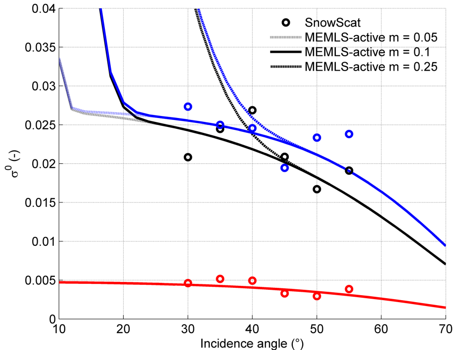
Figure 13. \sigma^0 measured by SnowScat (circles) and modeled by MEMLS3&a with CT input (lines) at 10.65 GHz for different mean slope of surface undulations m . The effect of m is limited to small incidence angles. Colors represent polarization, with vv – black, hh – blue and hv – red. Best fit parameters according to Fig. 8.
