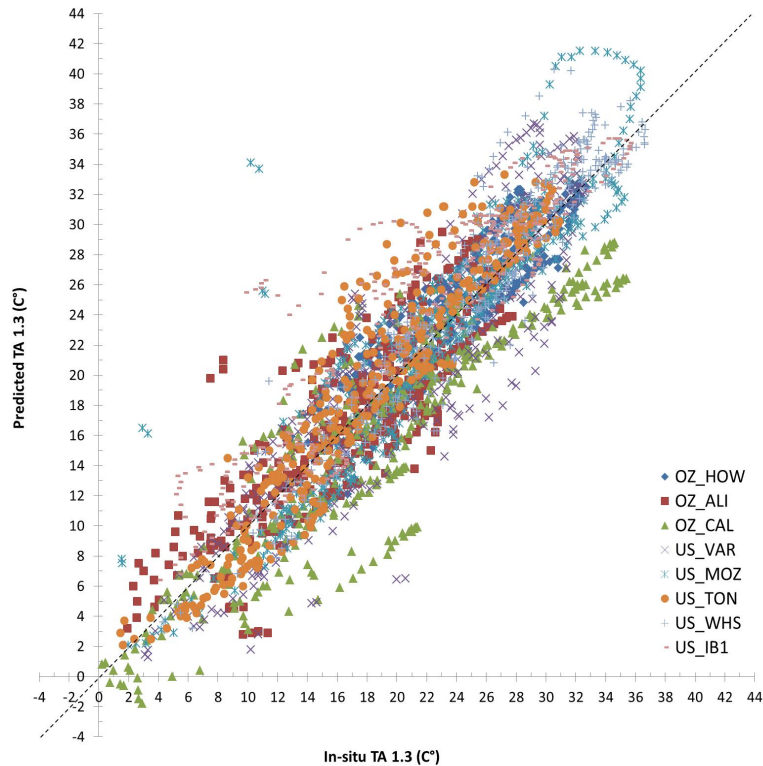
Figure 8. Scatterplot comparison of SimSphere predicted and in situ T_{air1.3m} .
