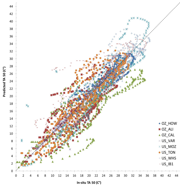
Figure 9. Scatterplot comparison of SimSphere predicted and in situ T_{air50m} .
