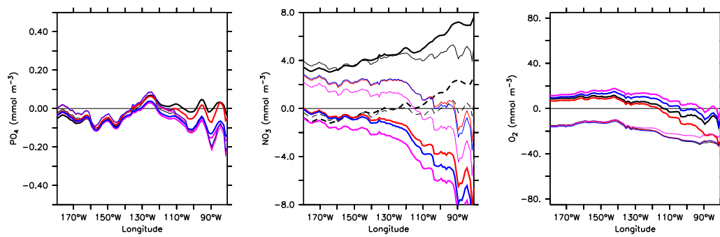
Figure 6. Phosphate (left), nitrate (middle) and oxygen (right) averaged over \pm 5^\circ and 0-6500 m, and plotted from 180^\circ\text{W} - 80^\circ\text{W} , for different models (lines) and observations (circles), plotted as difference to average observed concentrations. Black: model BUR (without nitrogen); nitrate is calculated from 16 \times phosphate (i.e. from the stoichiometry prescribed by the model; straight lines) as well as from 14.28 \times phosphate (i.e. from the global observed ratio; dashed lines). Red: MOPS, setup REFBASE, Pink: MOPS, setup DenHigh, Blue: MOPS, setup RemHigh. Thin lines denote model experiments with fast sinking speed, thick lines model experiments with slow sinking speed. Note that model axes for phosphate, nitrate and oxygen scale in a ratio of 1:16:170 (i.e., according to aerobic stoichiometry). See the discussion paper for a plot of absolute concentrations.
