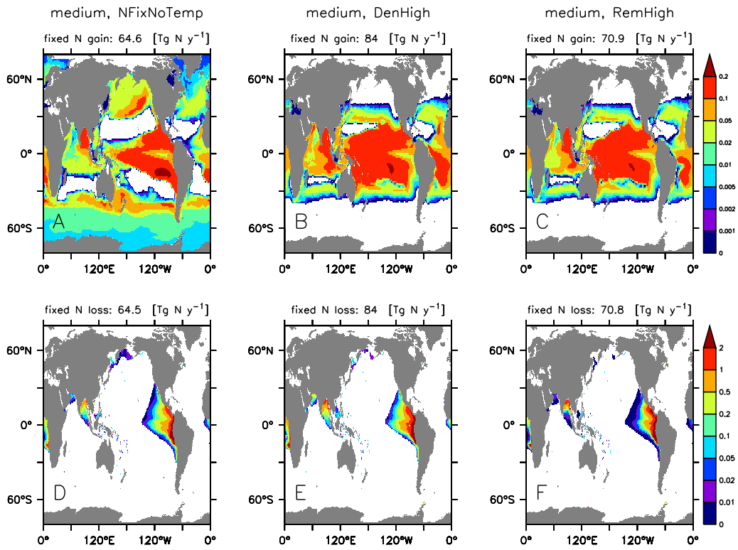
Figure 8. As figure 7, but for “medium” configuration of NFixNoTemp (no temperature dependence of nitrogen fixation, panels A, D), model setup DenHigh (high nitrate affinity of denitrification, panels B, E) and model setup RemHigh (high oxidant affinity of denitrification and aerobic remineralization, panels C, F).
