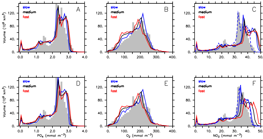
Figure 4. Volume distributions of global phosphate (panels A,D), oxygen (panels B, E) and nitrate (panels C, F) for model BUR of Krist and Oschlies (2013, upper panels A-C), and experiment REF BASE of MOPS (lower panels D-F). Grey bars denote the corresponding observations (Garcia et al., 2006a, b). Lines thickness Colors denotes different sinking speeds. ThickBlue: slow sinking. MediumBlack: medium sinking. ThinRed: fast sinking. Nitrate for model BUR (without nitrogen cycle) has been calculated from phosphate \times 16 . In addition, we present nitrate calculated from phosphate \times 14.28 for the “slow” sinking scenario as thick dashed red blue lines.
