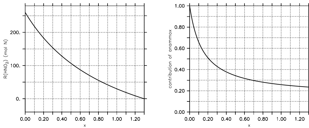
Figure 13. Nitrite surplus per mole of organic phosphorus remineralized (left), and contribution of anammox to fixed nitrogen loss (right) plotted vs. plotted against x , the ratio of nitrite reduction rate to nitrate reduction rate for denitrification combined with oxidation of ammonium by anammox. See text for further details.
