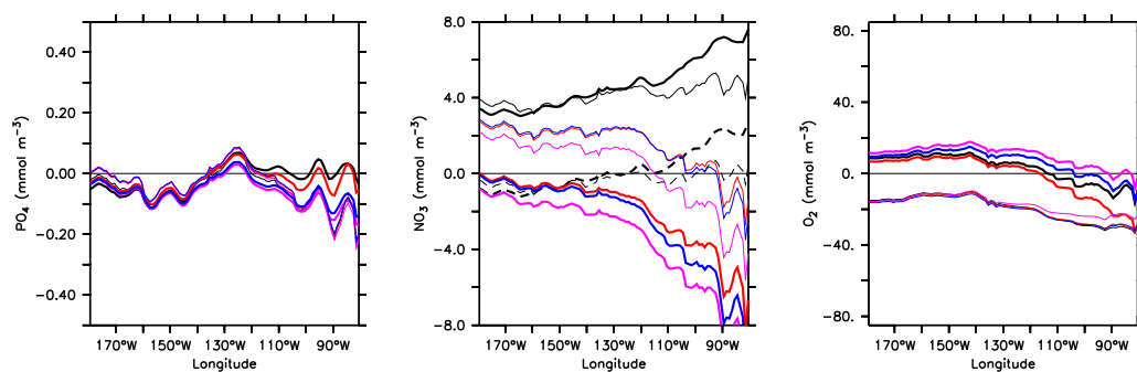
Figure 6. Phosphate (left), nitrate (middle) and oxygen (right) averaged over \pm 5^\circ and 0-6500 m, and plotted from 180^\circ\text{W} - 80^\circ\text{W} , for different models, plotted as difference to average observed concentrations. Black: model BUR (without nitrogen); nitrate is calculated from 16 \times phosphate (i.e. from the stoichiometry prescribed by the model; straight lines) as well as from 14.28 \times phosphate (i.e. from the global observed ratio; dashed lines). Red: MOPS, setup BASE, Pink: MOPS, setup DenHigh, Blue: MOPS, setup RemHigh. Thin lines denote model experiments with fast sinking speed, thick lines model experiments with slow sinking speed. Note that model axes for phosphate, nitrate and oxygen scale in a ratio of 1:16:170 (i.e., according to aerobic stoichiometry). See the discussion paper for a plot of absolute concentrations.
