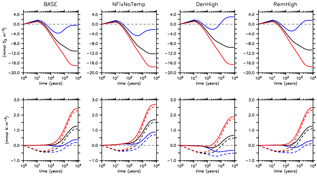
Figure 2. Transient behavior of global average oxygen (top), nitrate (bottom, dashed lines) and fixed nitrogen (bottom, straight lines) in different setups of model MOPS, plotted as deviation from initial average ( \bar{x}(t) - \bar{x}(0) ), where \bar{x} is either global average oxygen or nitrate). Average tracers are calculated from snapshots of day 360 every 10th year within the first 200 years, and every 100th year thereafter. Line colors denote different sinking speeds: Red - “fast”, black: “medium”, blue - “slow”. Model identifier is shown on top of each column. For better visibility on all timescales, we present the time axis on a logarithmic scale. Note that as models were started from observed global average tracers, any deviation from the dashed (zero) line also denotes the model bias.
