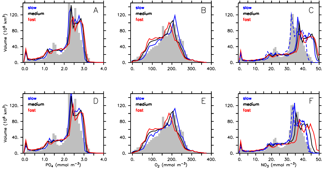
Figure 4. Volume distributions of global phosphate (panels A,D), oxygen (panels B, E) and nitrate (panels C, F) for model BUR of Krist and Oschlies (2013, upper panels A-C), and experiment BASE of MOPS (lower panels D-F). Grey bars denote the corresponding observations (Garcia et al., 2006a, b). Colors denotes different sinking speeds. Blue: slow sinking. Black: medium sinking. Red: fast sinking. Nitrate for model BUR (without nitrogen cycle) has been calculated from phosphate \times 16 . In addition, we present nitrate calculated from phosphate \times 14.28 for the “slow” sinking scenario as dashed blue lines.
