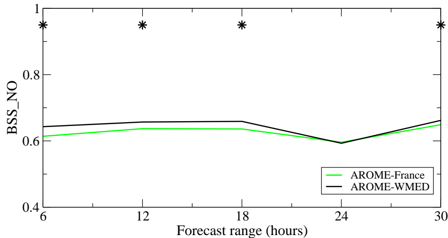
Figure 17. Brier skill score for simulated 10.8 \mu\text{m} SEVIRI brightness temperature lower than 240 K as a function of forecast range for SOP2 period (1 February 2013–15 March 2013). Stars indicate the statistical significance of the differences at a 90 % level.
