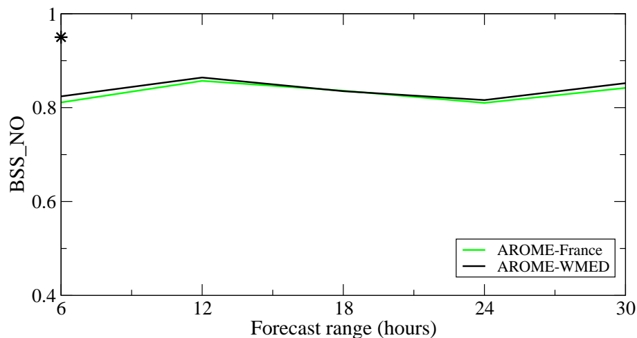
Figure 18. Brier skill score for 1 h wind gust exceeding 40 \text{ km h}^{-1} during the last hour as a function of forecast range during the SOP2 (1 February 2013–15 March 2013). Stars indicate forecast range where differences are statistically significant at a 90 % level.
