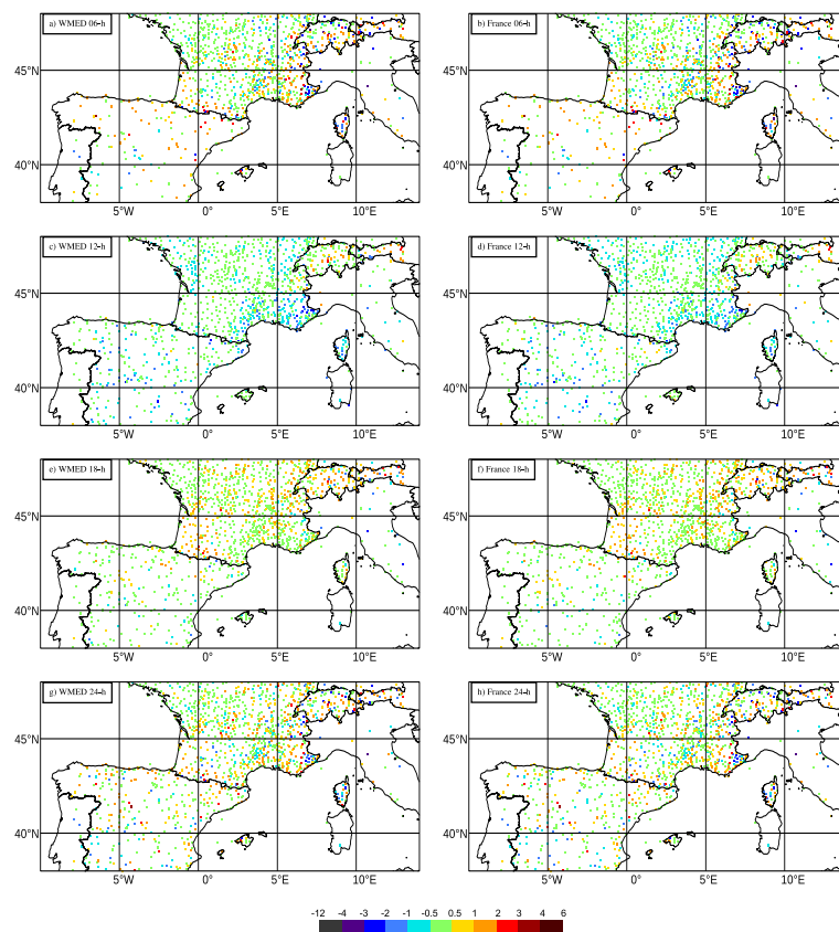
Figure 8. 2 m temperature bias (model–observation, in °C) computed with surface data for the 6, 12, 18 and 24h forecast ranges for the SOP1 period ranging from 7 September to 5 November 2012, for AROME-WMED (left) and for AROME-France (right).
