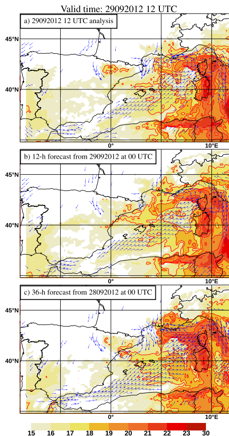
Figure 25. Wind at 925 hPa (blue arrows in excess of 20 \text{ m s}^{-1} ) and wet bulb temperature ( ^{\circ}\text{C} , colour scale) at 925 hPa from AROME-WMED analyses (a), 12 h (b) and 36 h (c) forecast ranges.
