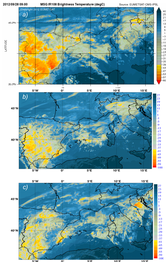
Figure 22. Brightness temperatures ( ^{\circ}\text{C} ) observed with SEVIRI on 28 September 2012 09:00 UTC (a) and simulated with AROME-WMED 9h forecast from 28 September 2012 00:00 UTC (b) and with 33 h forecast from 27 September 2012 00:00 UTC (c) .
