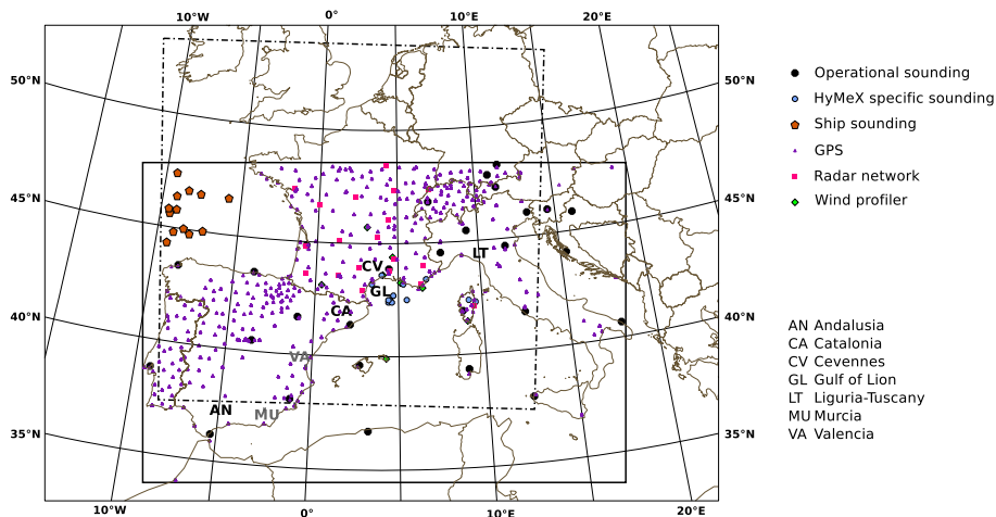
Figure 1. Location of various observation types assimilated in AROME-WMED model represented with symbols and domains of AROME-WMED (solid line box) and AROME-France (dashed dotted line box).
