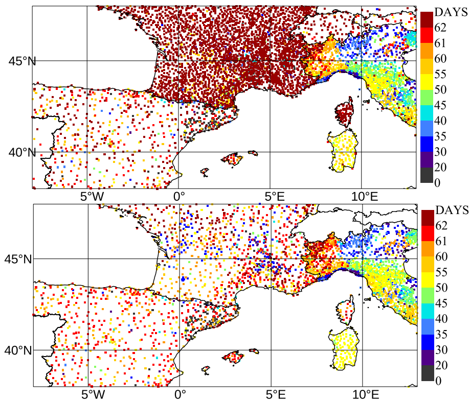
Figure 9. Number of available 24 h accumulated precipitation observations from 06:00 to 06:00 UTC next day (top) and from 00:00 to 00:00 UTC next day (bottom) for the period ranging from 5 September to 5 November 2012 (62 days) in the HyMeX database on 1 January 2014.
