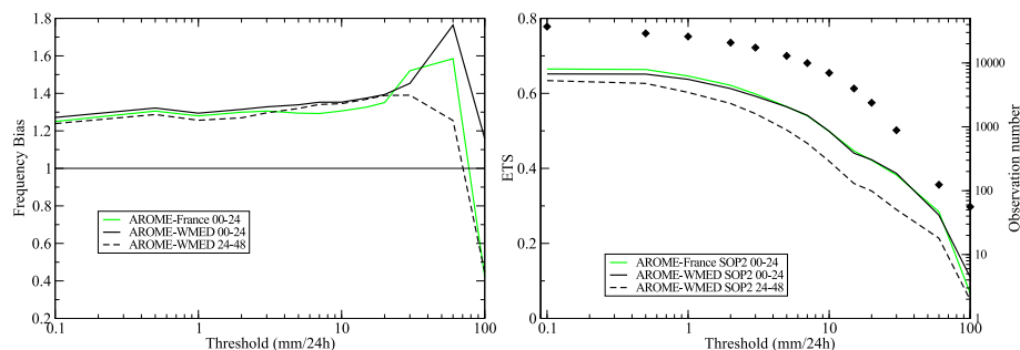
Figure 16. Frequency bias (left hand-side) and Equitable thread score (ETS, right hand-side) for the 0–24 h accumulated precipitation for AROME-France (green line) and AROME-WMED (black line) and for the 24–48 h accumulated precipitation for AROME-WMED (dashed black line) for the SOP2 periode from 1 February to 15 March 2013. Logarithm scale on x axis. Diamonds represent the number of observations used for the comparison (logarithm scale).
