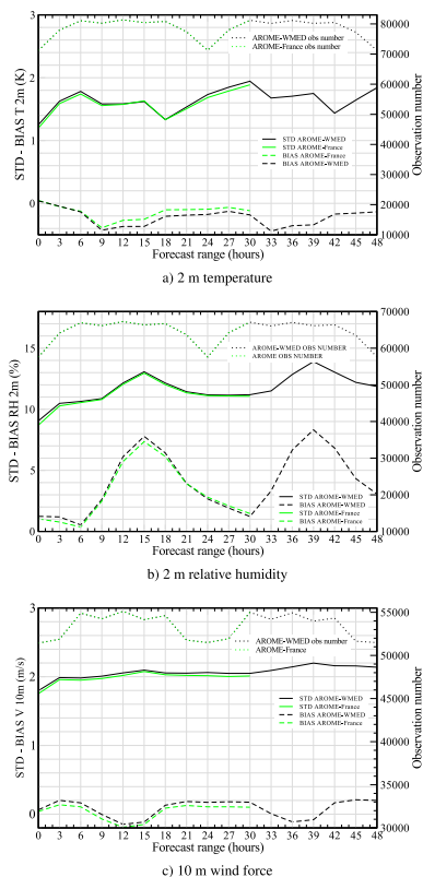
Figure 15. Bias (dashed lines) and standard deviation (solid lines) computed with 2 m temperature observations (a), 2 m relative humidity (b) and 10 m wind (c) with respect to the forecast range for the AROME-WMED model (black) and the AROME-France model (green) for SOP2 from 1 February to 15 March 2013. Dotted lines denote the number of observations used for the comparison (right y axis).
