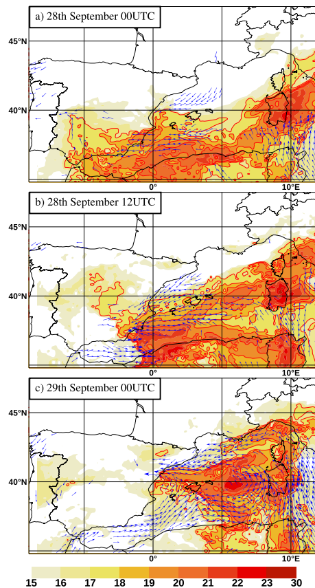
Figure 20. Wind at 925 hPa (blue arrows in excess of 20 \text{ m s}^{-1} ) and wet bulb temperature ( ^{\circ}\text{C} , colour scale) at 925 hPa from AROME-WMED analyses.
