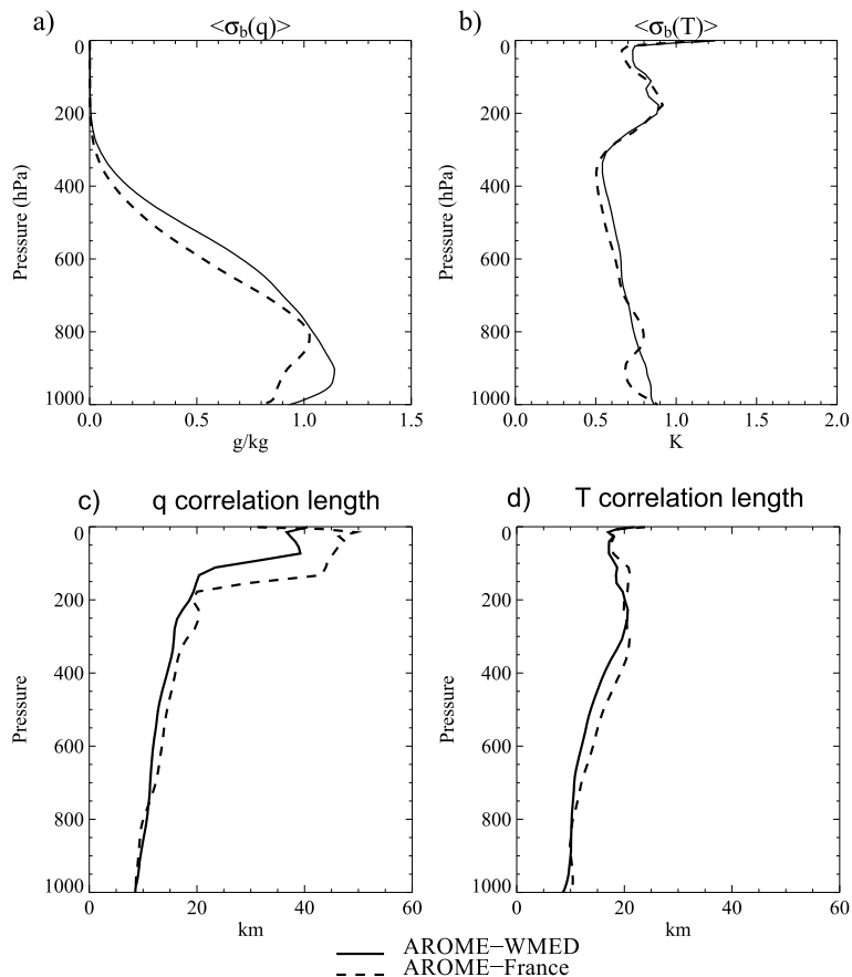
Figure 2. SD (a and b) and correlation length (c and d) of the AROME-WMED model (solid line) and of the AROME-France model (dashed line) for the humidity (left-hand panels) and the temperature (right-hand panels).
