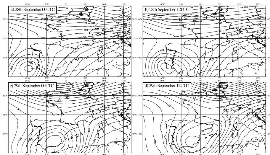
Figure 19. Geopotential height at 500 hPa (in dam) from operational ARPEGE analyses.
