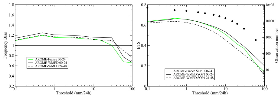
Figure 10. Frequency bias (left hand-side) and Equitable Threat Score (ETS, right hand-side) for the 0–24 h accumulated precipitation simulated by AROME-France (green line) and AROME-WMED (black line) and for the 24–48 h accumulated precipitation predicted by AROME-WMED (dashed black line) during the SOP1 period from 5 September to 6 November 2012. Logarithm scale on x axis. Diamonds represent the number of observations used for the comparison.
