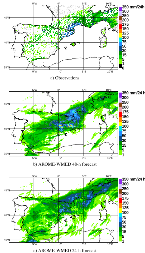
Figure 23. 24 h accumulated precipitation (mm) from 29 September 2012 at 00:00 UTC to 30 September at 00:00 UTC: observations (a) , 48 h AROME-WMED forecast (b) and 24 h AROME-WMED forecast (c) .
