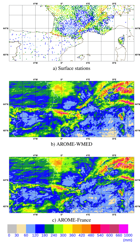
Figure 12. Accumulated precipitation (mm) during SOP1 period ranging from 5 September to 5 November 2012 measured by surface stations (Accumulation between 06:00 and 06:00 UTC next day, (a) predicted by AROME-WMED (b) and by AROME-France (c) ).
