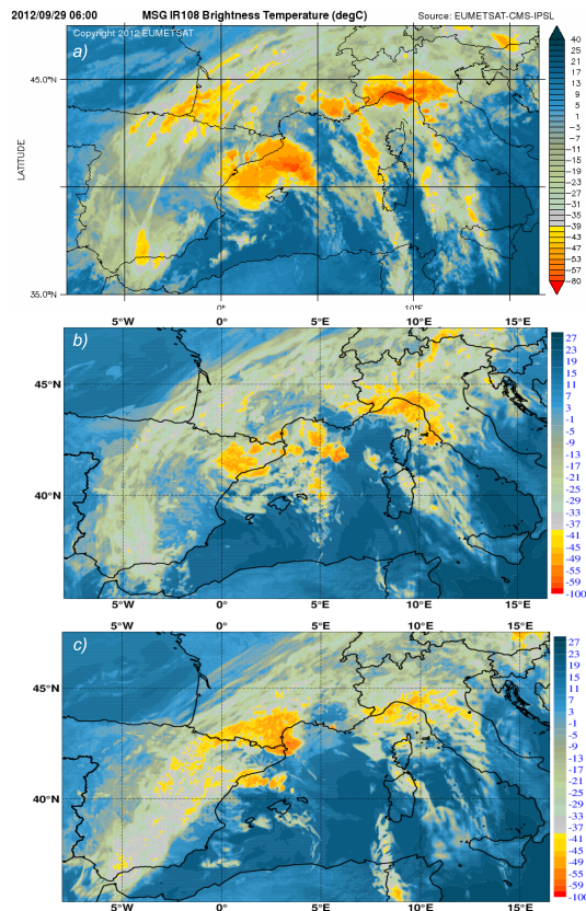
Figure 24. Brightness temperatures ( ^{\circ}\text{C} ) observed with SEVIRI on 29 September 2012 at 06:00 UTC (a) and simulated with AROME-WMED 6h forecast from 29 September 2012 00:00 UTC (b) and with 30 h forecast from 28 September 2012 00:00 UTC (c) .
