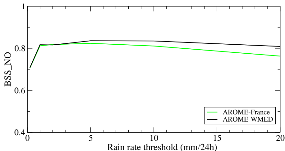
Figure 11. Brier skill score computed in a neighbouring distance of 54 km for AROME-France (green) and AROME-WMED (black) computed with raingauge data from France as a function of 6–30 h rain rate threshold during the SOP1 period from 5 September to 5 November 2012. Stars indicate the statistical significance of the differences at a 90 % level.
