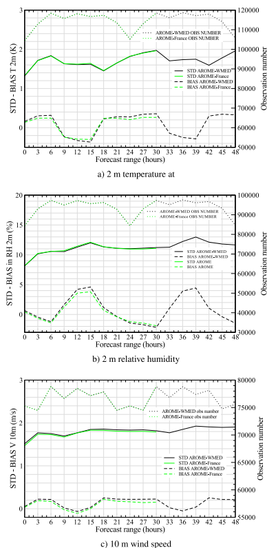
Figure 7. Bias (dashed lines) and SD (solid lines) computed with 2 m temperature (a) , 2 m relative humidity (b) and 10 m wind speed (c) with respect to the forecast range for the AROME-WMED model (black) and the AROME-France model (green) for SOP1 from 5 September to 6 November 2012. Dotted lines denote the number of observations used for the comparison (right y axis).
