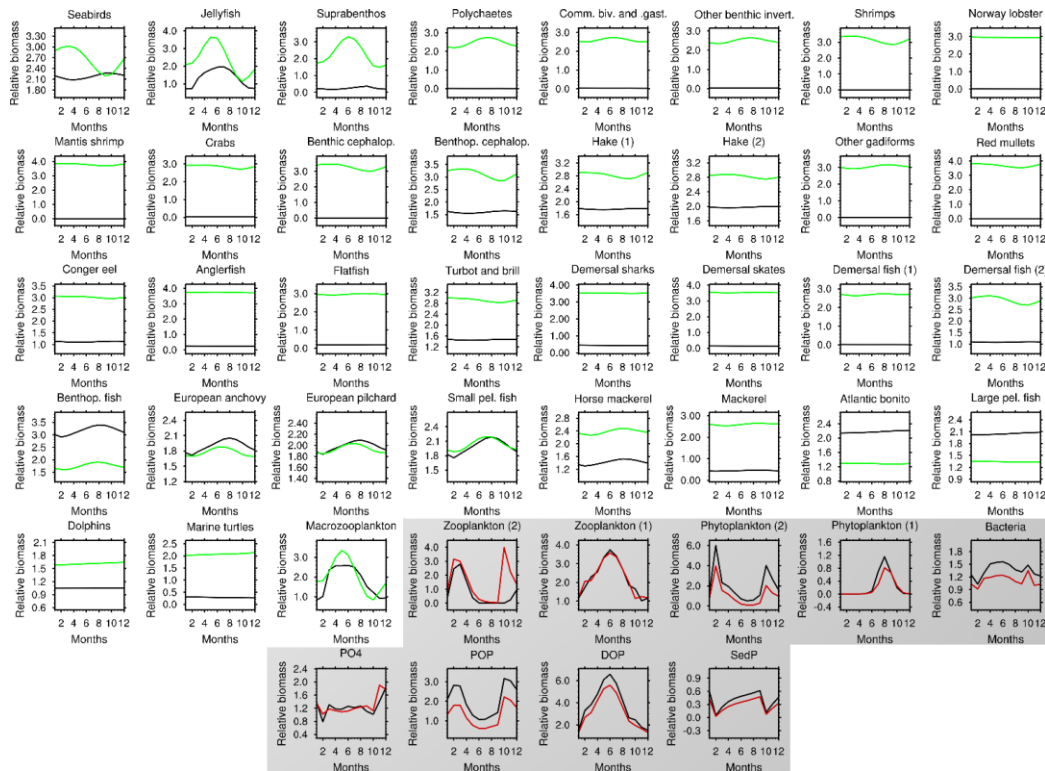
Figure 6. Monthly results of the final year in a 10-year simulation of the coupled (black lines) model versus simulations of uncoupled EwE (green lines for HTL variables – unshaded boxes) and uncoupled biogeochemical (red lines for grey shaded-LTL variables – grey shaded boxes) models.
