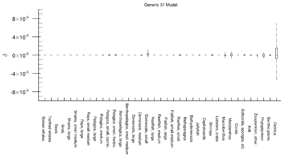
Figure 2. The residuals between absolute biomasses simulated by EwE 6.46.5 and EwE-F 1.0 for the Generic 37 model. X-axis denotes all state variables in the model.
