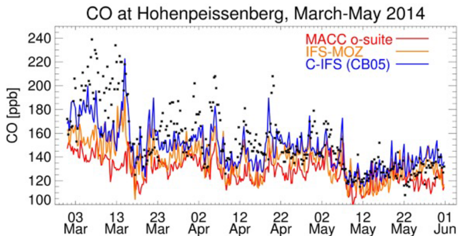
Figure 6. O-suite (red), stand-alone IFS-MOZART (orange) and C-IFS (CB05) (blue) compared to GAW observations (black dots) at Hohenpeissenberg station ( 47.80^{\circ} N, 11.02^{\circ} E) for the period March–May 2014.
