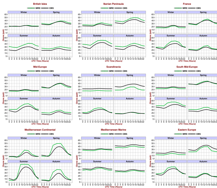
Figure 5. Mean 2003–2012 diurnal cycle of near surface ozone for the different European subregions based on MRE (green line) and observations (black line) calculated for winter (DJF), spring (MAM), summer (JJA) and autumn (SON).
