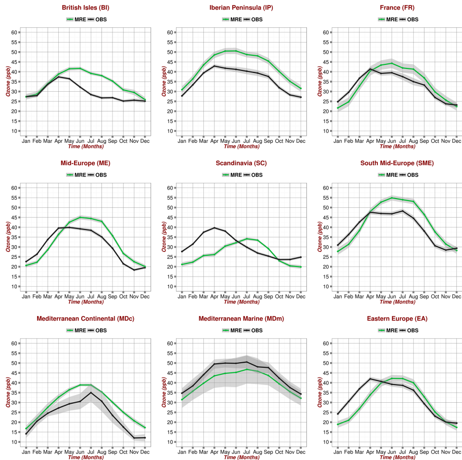
Figure 4. Mean 2003–2012 annual cycle of near surface ozone for the different European sub-regions of the MACC reanalysis and observations. The shading areas denote 95 % confidence interval of the mean values.
