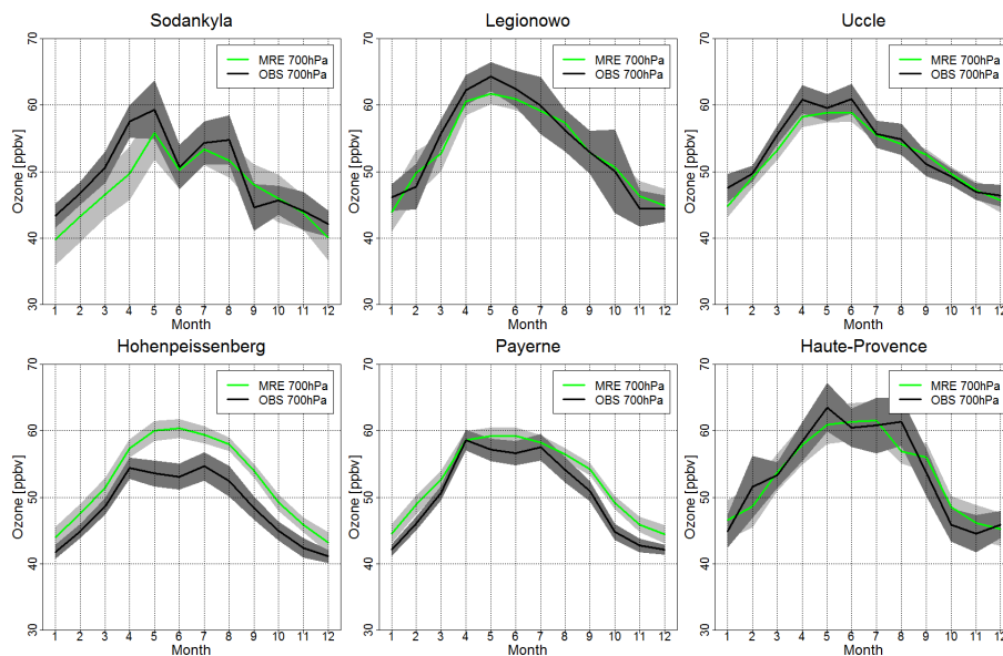
Figure 8. Mean 2003–2012 annual cycle of near surface ozone at 700 hPa based on MRE (green line) and ozonesonde measurements (black line) at the stations of Sodankyla (67.4° N, 26.6° E), Legionowo (52.4° N, 20.9° E), Uccle (50.8° N, 4.3° E), Hohenpeissenberg (47.8° N, 11° E), Payerne (46.8° N, 6.9° E), and Haute-Provence (43.9° N, 5.7° E). The shading areas denote 95 % confidence interval of the mean values.
