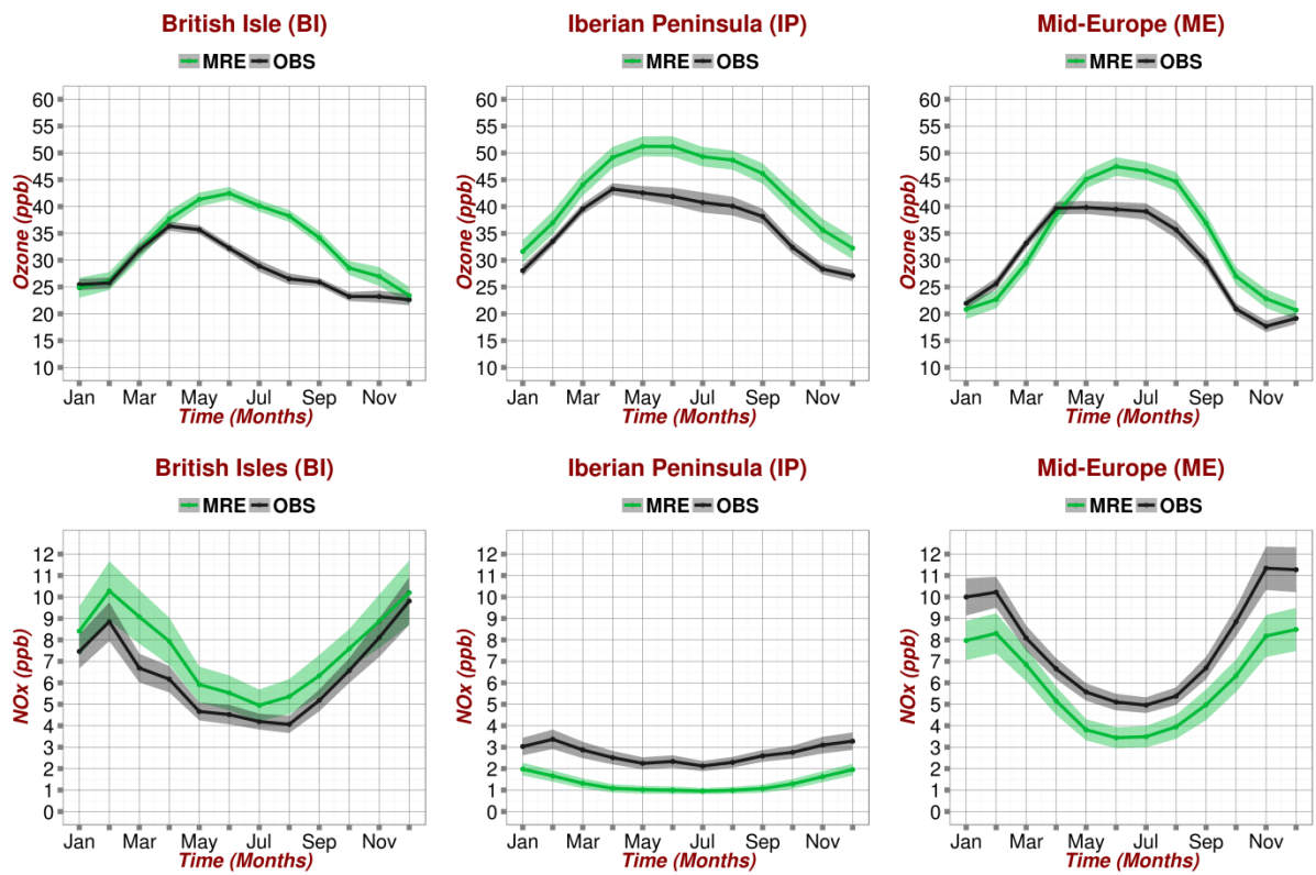
4 Figure 9. Mean annual cycle of near surface O 3 (top panel) and NO x (bottom panel) based on 5 observations (solid black line) and MRE (green line) for the subregions BI, IP, ME over the 6 period 2003-2012.
