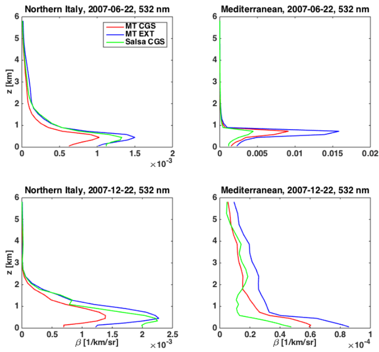
Figure 11. Backscattering coefficient at a wavelength of 532 nm at Northern Italy and Mediterranean and at two different time events (22/6 and 22/12-2007 at 12.00), computed with the three model versions, MT-EXT (blue), MT-CGS (red) and Salsa-CGS (green).
