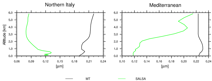
Figure 7. Effective radius, r_{eff} , for the two chemical transport model versions MT and SALSA over Northern Italy and Mediterranean the 2007-06-22 at 12:00.
