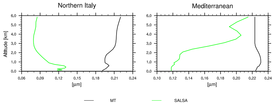
Figure 7. Effective radius, r_{\text{eff}} , for the two chemical transport model versions MT and SALSA over Northern Italy and Mediterranean the 2007-06-22 at 12:00.
