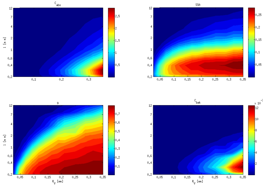
Figure 2. Absorption cross section C_{abs} (upper left), single-scattering albedo SSA (upper right), asymmetry parameter g (bottom left), and backscattering cross section C_{bak} (bottom right) of black carbon aggregates as a function of volume-equivalent radius R_V and wavelength \lambda .
