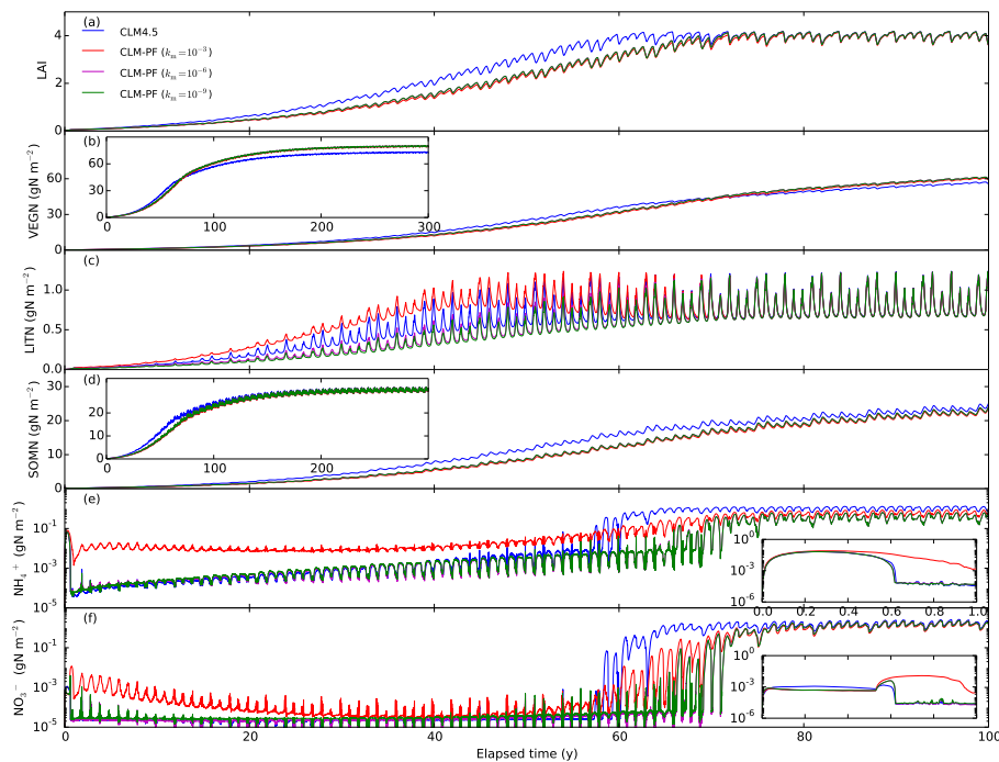
Figure 6. Calculated LAI and nitrogen distribution among vegetation, litter, SOM, \text{NH}_4^+ , and \text{NO}_3^- pools in spin-up simulations for BR-Cax site.
