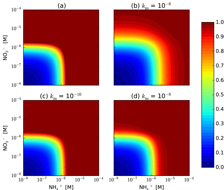
Figure 3. f_{pi} = \frac{N_{take}}{N_{demand}} = \max\left(1, \frac{[NH_4^+] + [NO_3^-]}{N_{demand}}\right) (a) vs. = \frac{[NH_4^+]}{k_m + [NH_4^+]} + \left(1 - \frac{[NH_4^+]}{k_m + [NH_4^+]}\right) \frac{[NO_3^-]}{k_m + [NO_3^-]} (b–d) in a 0.5 h time step with an uptake rate of 10^{-9} \text{ Ms}^{-1} . f_{pi} for the latter representation is less than or equal to that for the first one. The difference decreases with decreasing half saturation k_m .
