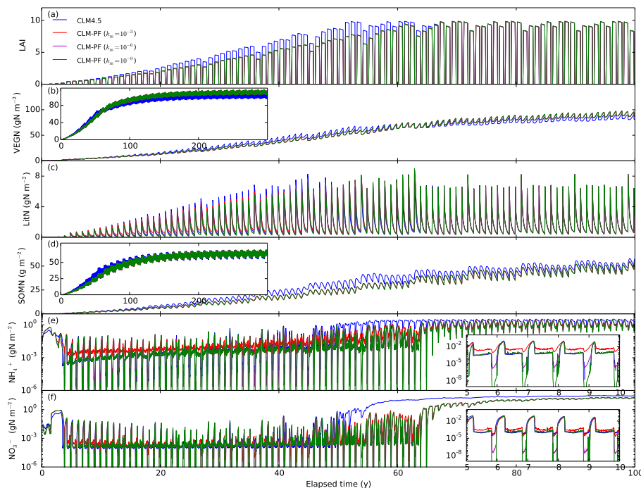
Figure 5. Calculated LAI and nitrogen distribution among vegetation, litter, SOM, \text{NH}_4^+ , and \text{NO}_3^- pools in spin-up simulations for US-WBW site.
