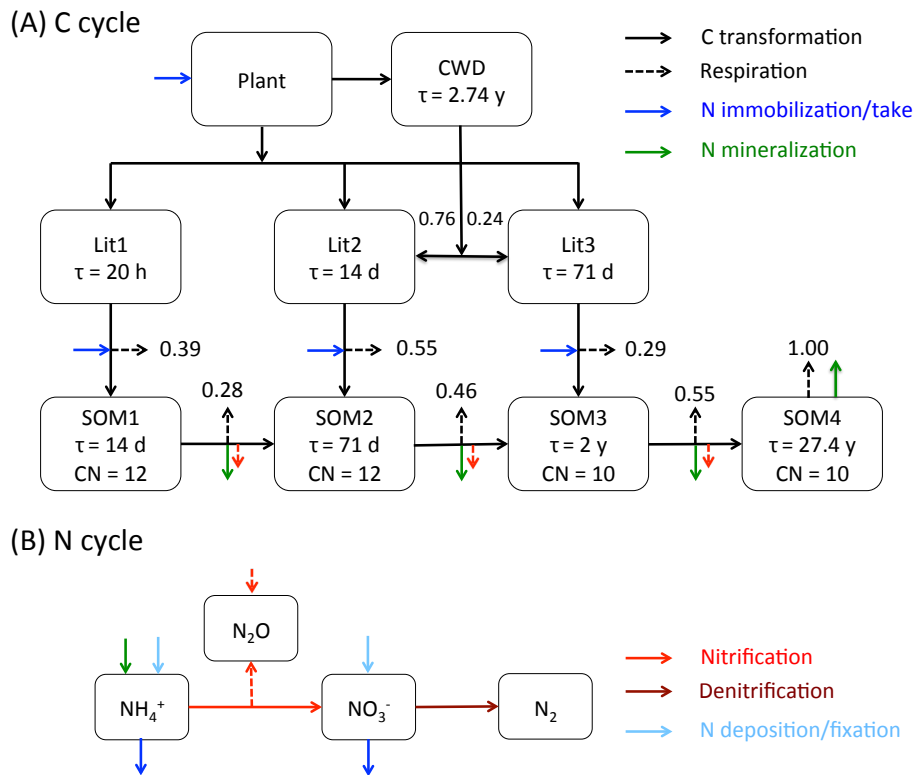
Figure 1. The reaction network for the carbon (A) and nitrogen (B) cycles implemented in this work. The carbon cycle is modified from Thornton and Rosenbloom (2005) and Bonan et al. (2012). \tau is the turnover time, and CN is the CN ratio in g C over g N.
