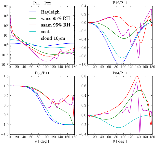
Fig. 3. Phase matrix elements for the basic OPAC aerosol types “water soluble” ( waso ), “sea salt accumulated mode” ( ssam ), and soot , for a water cloud with a droplet effective radius of 10 \mu\text{m} , and for Rayleigh scattering (with \delta=0 ) at a wavelength of 350 \text{ nm} . \theta is the scattering angle, i.e. the angle between incoming and scattered directions.
