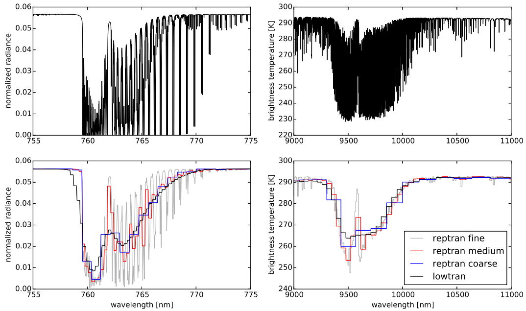
Fig. 2. Nadir top of the atmosphere radiance in the oxygen-A band around 760 nm (left) and in the IR window region (right) for the midlatitude-summer atmosphere of Anderson et al. (1986). All calculations were performed with the MYSTIC solver using the “absorption lines importance sampling” method (Emde et al., 2011). (Top) High spectral resolution calculation, based on line-by-line absorption cross sections calculated using ARTS (Eriksson et al., 2011); (bottom) pseudo-spectral calculations using the representative wavelengths band parameterizations ( reptran ) with different resolutions and lowtran . For comparison see also Fig. 3 in Mayer and Kylling (2005) which shows transmittances for genln2 line-by-line calculations and lowtran for the same spectral regions.
