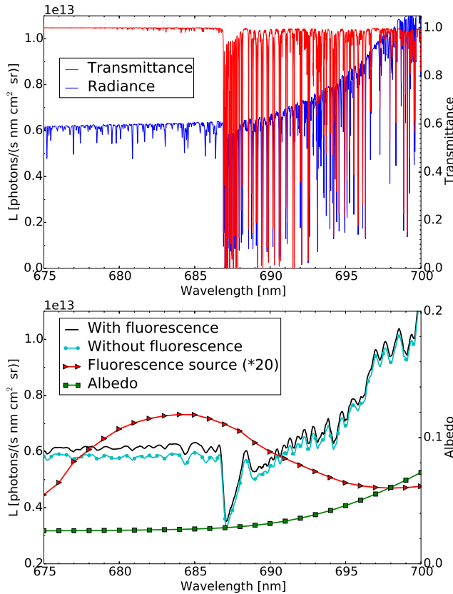
Fig. 7. (Upper plot) The transmittance from ARTS output and radiance from uvspec . (Lower plot) The top of the atmosphere nadir viewing radiance in the O 2 -B band with (blue-black line) and without (purple-cyan line with circles) a surface fluorescence source (red line with triangles). The radiances have been convolved with a spectral response function with FWHM of 0.3 nm.
