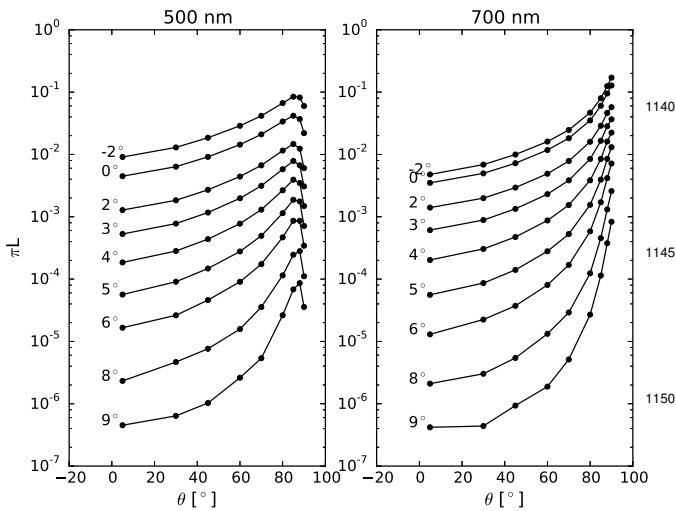
Fig. 11. Twilight radiance at 500 nm and 700 nm calculated using fully spherical geometry for the US-standard atmosphere. The lines are for different solar depression angles. The x-axis corresponds to the viewing zenith angle.
