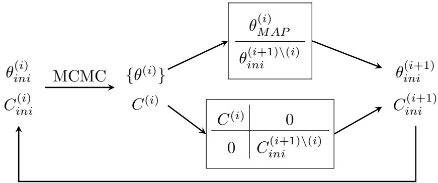
Figure 11. Schematic of the iterative process for parameter calibration. The MCMC sampling of the joint density for the set of parameters \theta^{(i)} starts at \theta_{ini}^{(i)} using an initial proposal covariance C_{ini}^{(i)} . For the following iteration, (i + 1) , the initial condition is constructed using the MAP estimate for \theta^{(i)} , augmented with initial conditions, in this case the nominal values, for the rest of parameters, \theta^{(i+1)\setminus(i)} . The initial proposal covariance C_{ini}^{(i+1)} is constructed based on the sample covariance matrix for \theta^{(i)} , augmented with an initial proposal covariance for \theta^{(i+1)\setminus(i)} , C_{ini}^{(i+1)\setminus(i)} .
