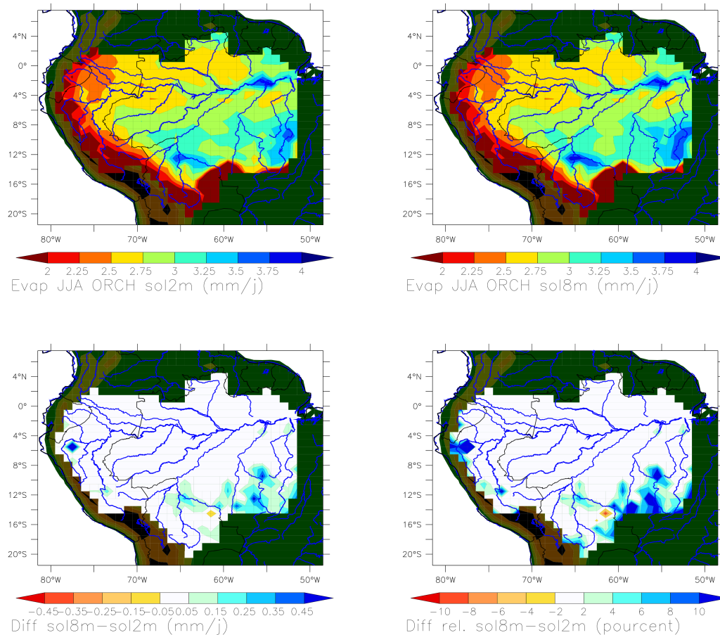
Fig. 1. Test of soil depth impact on JJA ET with the 11LAY, over the Amazon basin.
