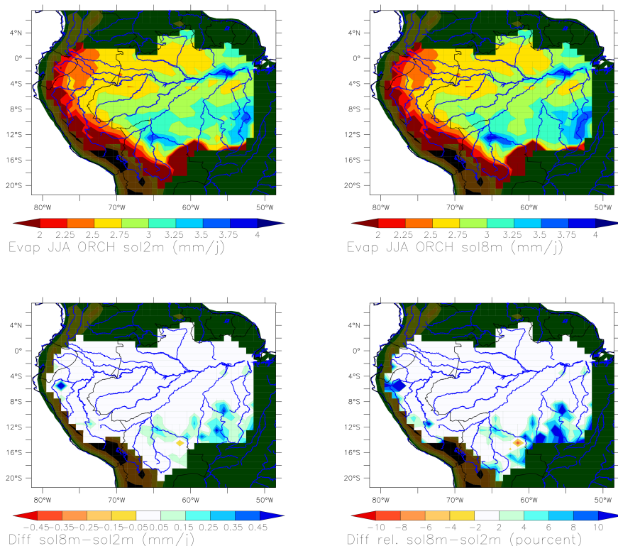
Fig. 1. Test of soil depth impact on JJA ET with the 11LAY, over the Amazon basin.
