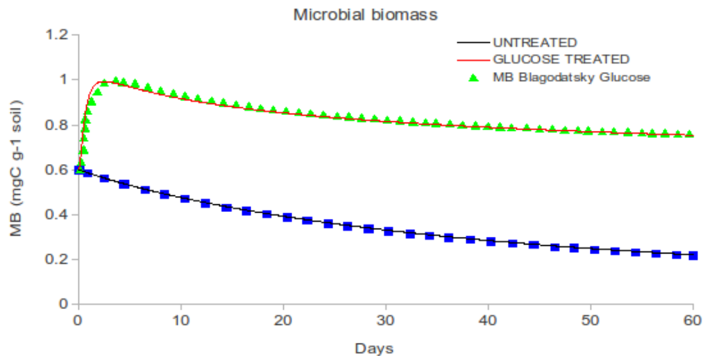
Fig. 3. Microbial biomass for 60 days from the start of the experiment. Lines are the DecoBio model and points are data from Blagodatsky et al. (2010).
