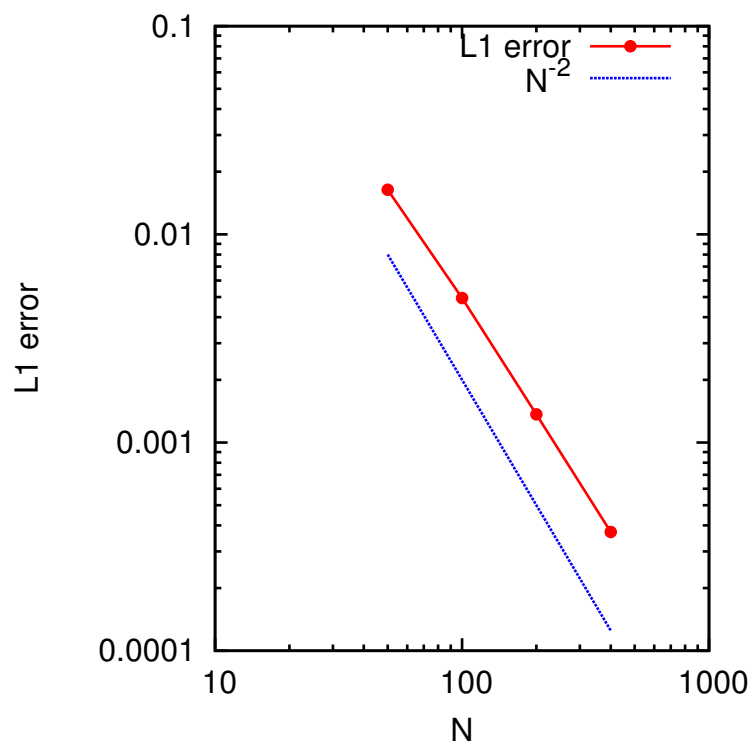
Fig. 2. L1 error norm for different grid spacings.
