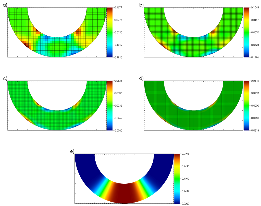
Fig. 1. Difference tracer field after one rotation for a) N=50, b) N=100, c) N=200, d) N=400, e) Tracer field after one rotation for N=400.
