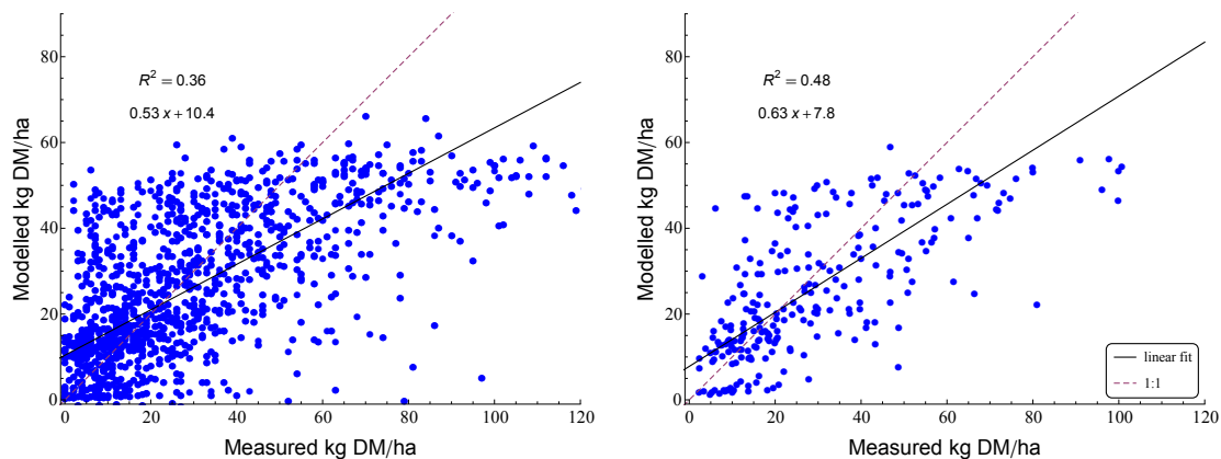
Fig. 2. Scatter plot of modelled vs. measured pasture growth for validation sites. (Fig. 4 in manuscript)
