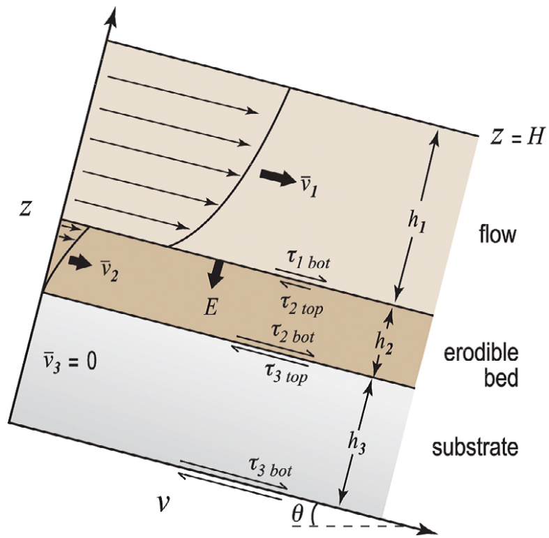
Fig. 1. Figure 1. Schematic illustration of velocity profiles (Iverson, 2012)
