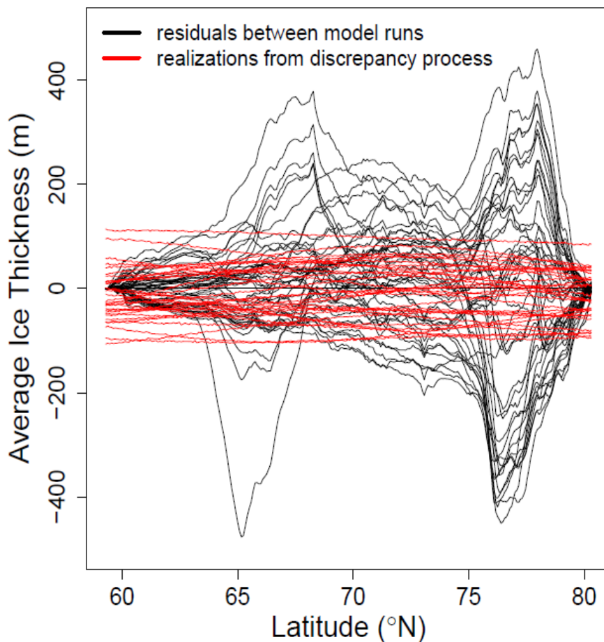
Fig. S1 Comparison between (i) residuals between the synthetic truth used in the main text (model run #67 in Applegate et al.) and other model runs (black solid curves) and (ii) 30 different realizations from the model for the simulated discrepancy (red solid curves). The residuals are computed by subtracting
