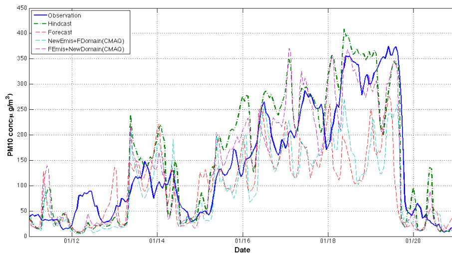
Fig. 5. The time series of the PM 10 hourly concentration during the air pollution episode in January 2010. The “added” cyan dashed line is only updated emissions, and magenta dashed only expanded domain.
