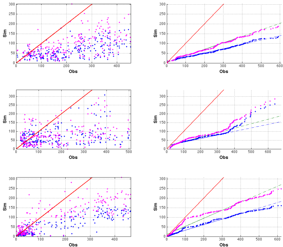
Fig. 2. The scatter plot and quantile–quantile (Q–Q) plots of the observed and simulated PM10 hourly concentration. The upper is Baoding, the middle is Tangshan, the lower is Xianghe.
