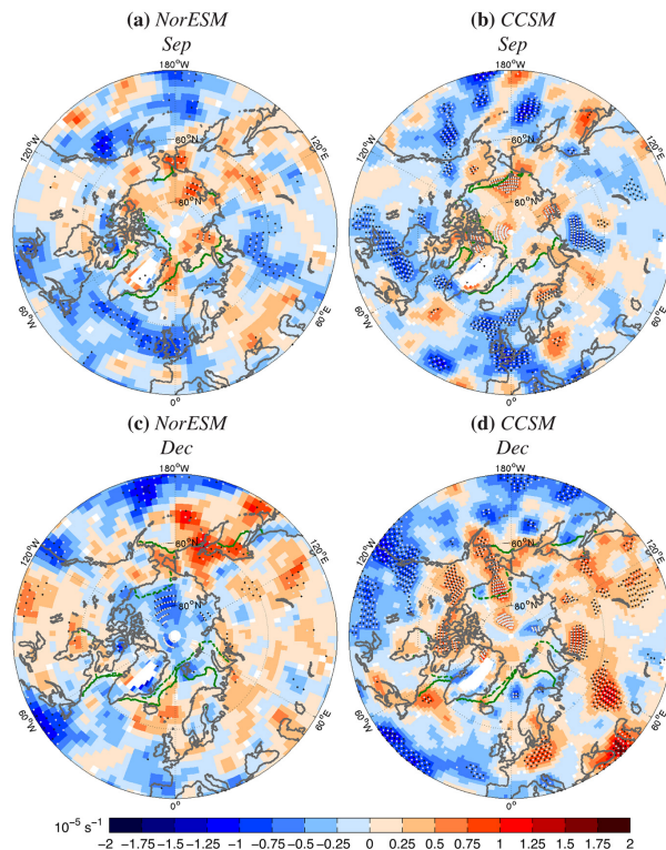
Figure 7. Average mean intensities for September (upper row) and December (lower row) 2074–2100 relative to 1979–2005 for the RCP8.5 scenario in (a), (c) NorESM and (b), (d) CCSM. Regions with track density below 0.5 \text{ no. density (month)}^{-1} (10^6 \text{ km}^2)^{-1} in the historical time period are shaded white. Alternating black and white dots mark regions where p < 0.05 based on 2000 samples. Solid and dashed green lines show the sea ice boundaries in each model and month over 1979–2005 and RCP8.5 2074–2100, respectively, calculated using a threshold of 15 % SIC.
