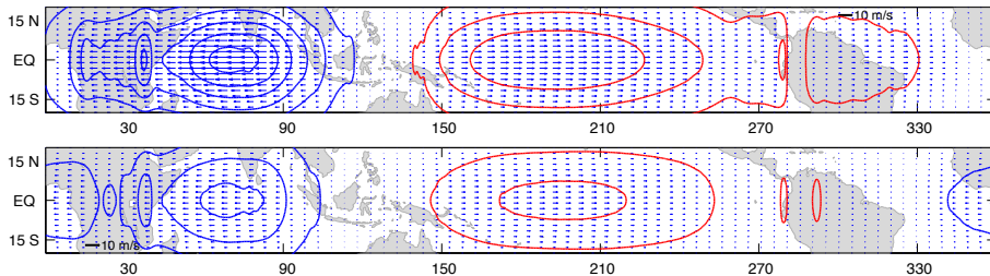
Figure 16. ERA-Interim climatology of Climatological Kelvin wave winds and geopotential height perturbations in ERA Interim for July on (upper panel) model level 27, at about 133 hPa and (panel below) and model level 31, at about 229 hPa. Isolines for the geopotential height are drawn every 10 m, starting from \pm 10 m with positive values in red and negative in blue.
