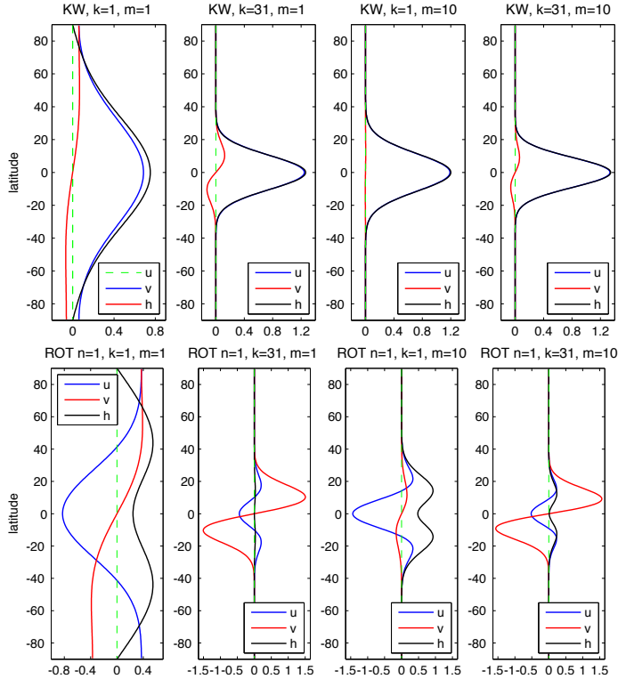
Figure 5. Meridional structure of the Hough harmonics for (top) Kelvin mode and (bottom) n = 1 balanced mode. Four The four panels for each mode correspond to various combinations of the zonal wavenumber k and vertical mode m , as defined in each panels' title.
