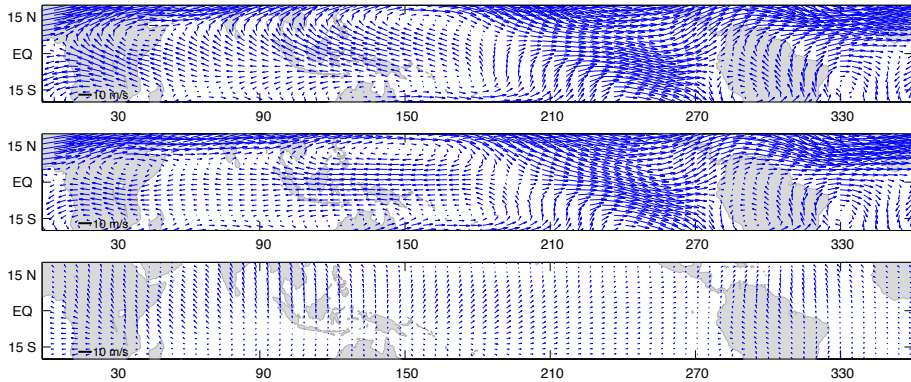
Figure 12. ERA-Interim Climatological horizontal winds in January on ERA Interim model level 31 (about 229 hPa) for (top) the total circulation, (middle) balanced circulation and (bottom) unbalanced circulation. Wind vectors in all panels are scaled by the same factor and drawn every \frac{3}{7} grid points in the zonal and meridional directions, respectively.
