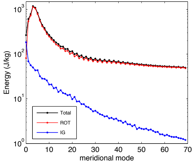
Figure 8. Distribution of total, balanced and inertio-gravity wave energy in meridional modes. Summation is performed over all (m, k) and the mean state ( k = 0 ) is not included.
