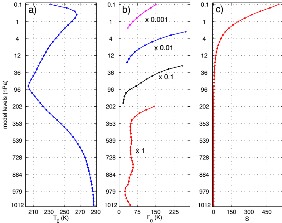
Figure 2. Globally-averaged vertical profiles of (a) temperature T_0 , (b) stability \Gamma_0 and (c) normalized stability parameter S on model levels which. The stability profile is input to the vertical structure equation (10). Profiles are based on ERA Interim model-level data for year 2000. Labels on y axis are average pressures of the model levels. Values of stability at various levels in (b) are scaled by different factors for clarity reasons. Under 200 hPa stability is not sealesscaled.
