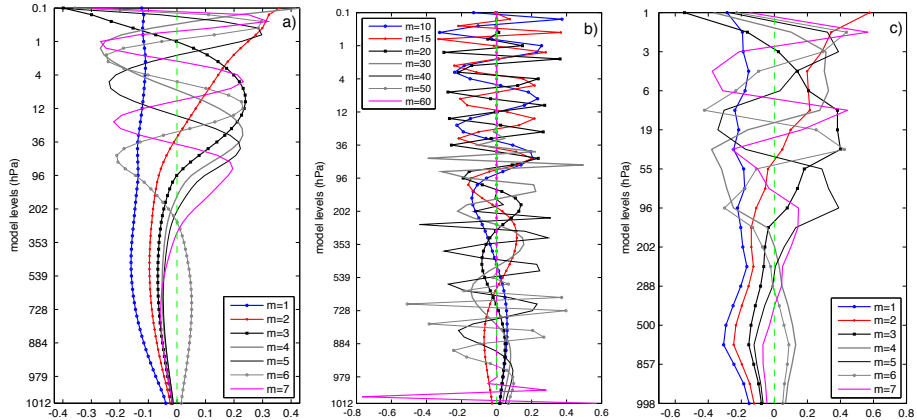
Figure 4. Vertical structure functions for (a) the first seven vertical modes and (b) modes 10, 15, 20, 30, 40 50 and 60, derived for using the 60 model levels of ERA Interim; (c) As Same as (a) but for the case of 21 model levels closest to the standard 21 pressure levels.
