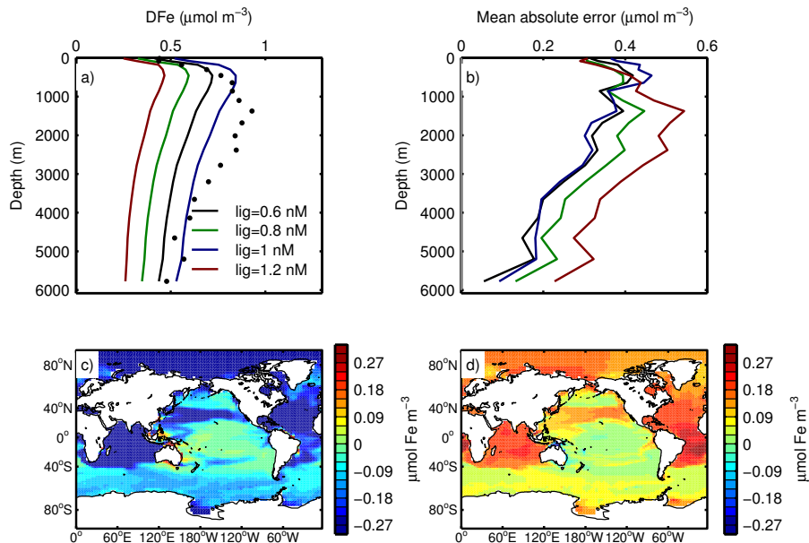
Figure 17. Impact of setting varying the iron solubility in dust to a globally constant value ligand concentration on the globally averaged vertical profiles of 1. (a) Annual mean simulated surface dissolved iron concentrations with observations compiled by plotted as colored circles on top (a), vertical profiles of the horizontally averaged absolute differences between model and the observations (b), difference of the between annual mean surface phosphate concentrations after 1000 with the dissolved iron solubility in dust concentrations when ligands are set to a at constant value values of 1 to the lig=0.6 nM and lig=1.0 nM (c), difference between annual mean surface phosphate dissolved iron concentrations when ligands are set at constant values of the standard simulation lig=1.2 nM and lig=1.0 nM (d).
