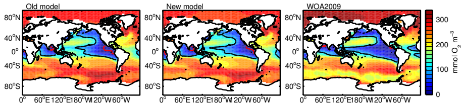
Figure 10. Annual mean oxygen concentrations at 450 m depth for the old model by Keller et al. (2012) and the new model in comparison to observations from the World Ocean Atlas 2009 (WOA, 2009) (García et al., 2010a). The black contour line is located at concentrations of 100 \text{ mmol O}_2 \text{ m}^{-3} , the red contour line is located at concentrations of 5 \text{ mmol O}_2 \text{ m}^{-3} .
