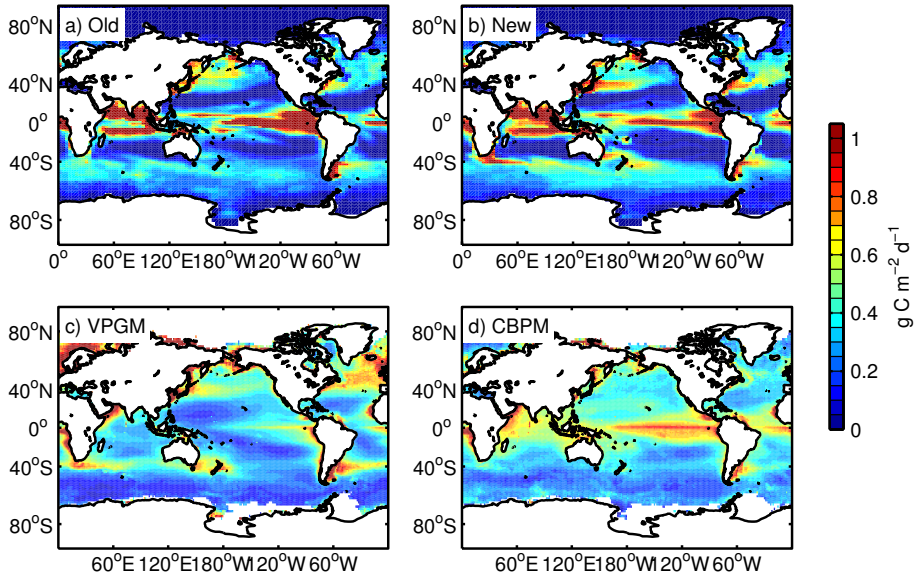
Figure 11. Marine vertically integrated annual mean net primary production for (a) the old model by Keller et al. (2012) (b) the new model with the dynamic iron cycle, (c) the vertically generalized production model (VPGM) by Behrenfeld and Falkowski (1997) and (d) the carbon-based productivity model (CBPM) by Westberry et al. (2008).
