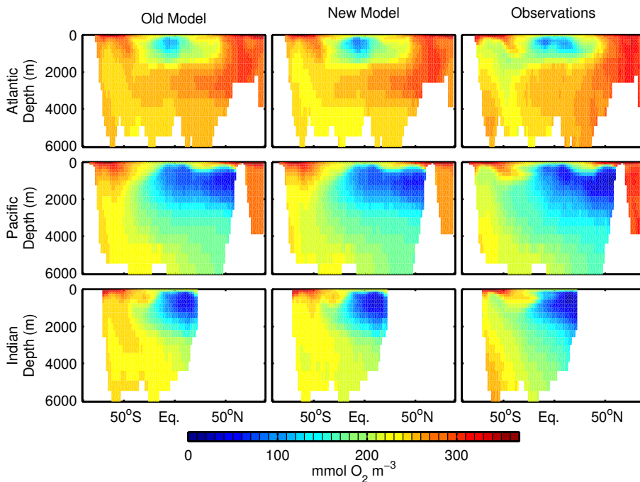
Figure 14. Zonal annual mean oxygen concentrations as simulated with the old model by Keller et al. (2012) (left column) and the new model (middle column) in comparison to observations from the World Ocean Atlas 2009 (WOA, 2009) (Garcia et al., 2010a) (right column) for the different ocean basins.
