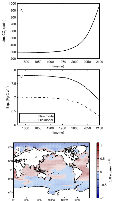
Figure 21. Results of the global warming scenario run following the high CO 2 emissions representative concentration pathway (RCP 8.5) scenario: (a) Annual average CO 2 concentrations with the new model and old-with-the-model-by Keller et al. (2012) (not distinguishable), (b) globally integrated export production at 80 m with the new model and old-with-the-model-by Keller et al. (2012), (c) the difference in surface dissolved iron concentrations between the year 2100 and year 1765.
