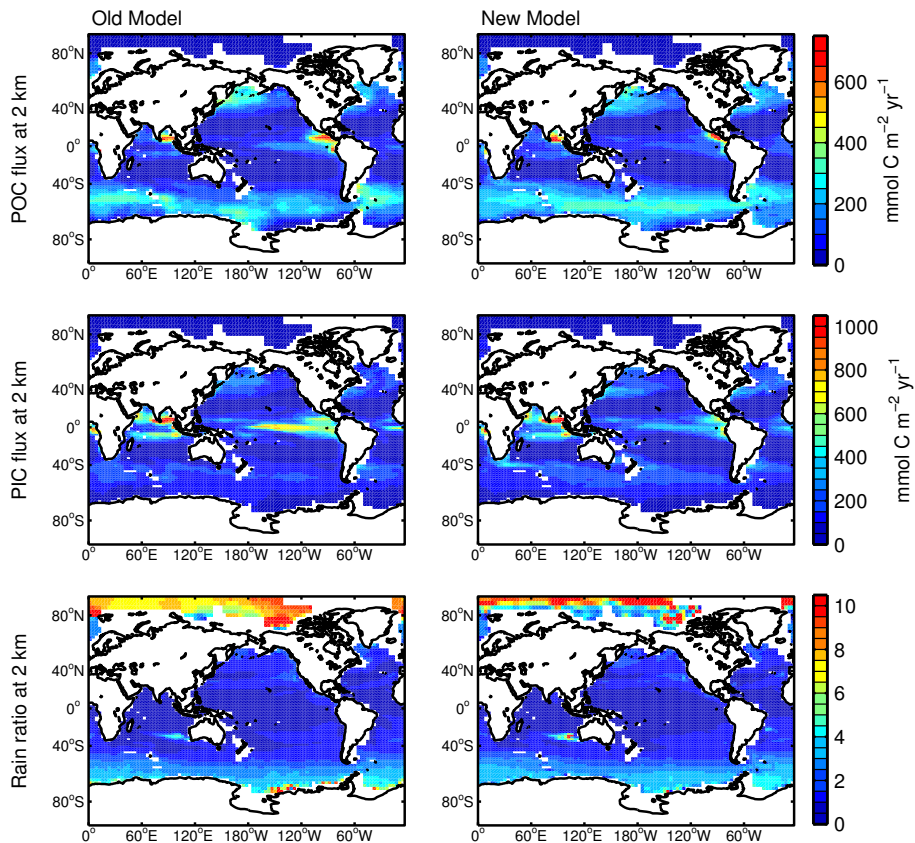
Figure 12. Annual fluxes of POC and PIC at 2 km and the rain ratio as simulated with the old model by Keller et al. (2012) (left column) and with the new model (right column).
