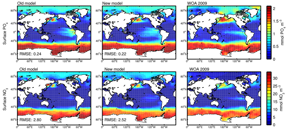
Figure 8. Annual mean surface phosphate (first row) and nitrate concentrations (second row) for the old model by Keller et al. (2012) and the new model in comparison to observations from the World Ocean Atlas 2009 (WOA, 2009) (Garcia et al., 2010b).
