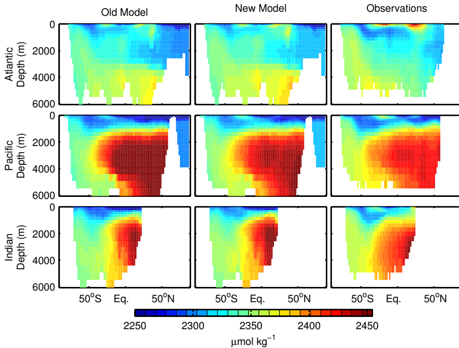
Figure 15. Zonal annual mean alkalinity as simulated with the old model by Keller et al. (2012) (left column) and the new model (middle column) in comparison to observations from GLODAP (right column) for the different ocean basins.
