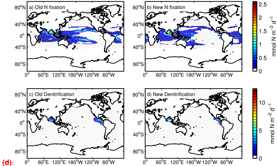
Figure 16. Annual mean nitrogen fixation with the model by Keller et al. (2012) (a) and the new model (b) and denitrification with the model by Keller et al. (2012) (c) and the new model (d). Values below 0.1 mmol N m -2 d -1 are not shown for (a) and (b) while values below 0.5 mmol N m -2 d -1 are not shown for (c) and (d).
