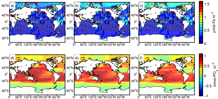
Figure 19. Impact of shutting of the subgridscale bathymetry after a 1000 year simulation. (a) Annual mean simulated surface iron concentrations with the subgridscale bathymetry shut off with observations compiled by Tagliabue et al. (2012) averaged over the first 50 m plotted as colored circles on top and for experiment BAT08 are shown in (a), for BAT10 in (b) and for BAT12 in (c) (cf. 2). The difference of between the annual mean surface phosphate concentrations with the subgridscale bathymetry shut off to the phosphate concentrations after 1000 years of the standard simulation experiment BAT08 and LIG08 are shown in (d) , between BAT10 and LIG10 in (e) and between BAT12 and LIG12 in (f) . The experiments are listed in Table 2.
