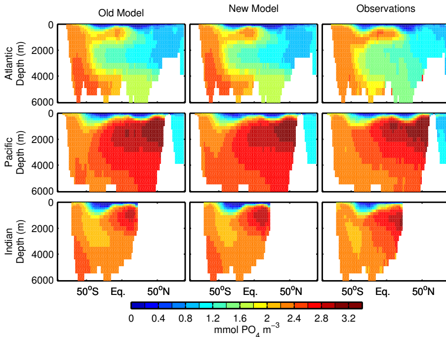
Figure 13. Zonal annual mean phosphate concentrations as simulated with the old model by Keller et al. (2012) (left column) and the new model (middle column) in comparison to observations from the World Ocean Atlas 2009 (WOA, 2009) (Garcia et al., 2010b) (right column) for the different ocean basins.
