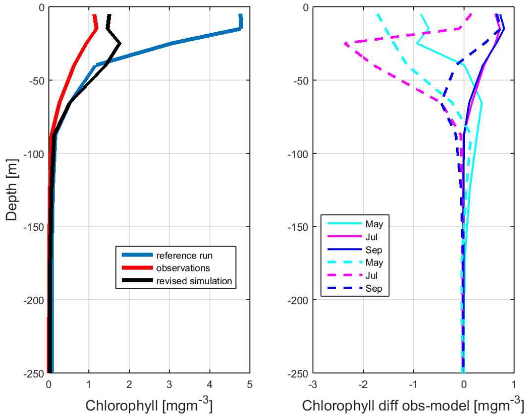
2 Figure 11. Chlorophyll profiles from the control and reference run using the higher resolution 3 model in June (a) in the Norwegian Sea box as well the difference between observations and 4 model in other months (b) – solid lines are the revised simulation and dashed lines the control 5 run. All observations in the Norwegian Sea box between 1998 and 2001 have been used.
