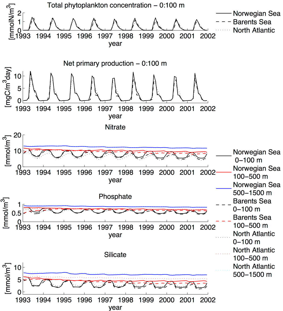
1 2 Figure 3. The temporal evolution of total phytoplankton, net primary production, and for the 3 three nutrients in different depth intervals from initialization in 1993 to the end of 2001. 4 Norwegian Sea and Barents Sea are here the boxes shown in Fig. 1. North Atlantic here 5 refers to the area from 80^\circ W to 80^\circ E and 60^\circ N to 80^\circ N
