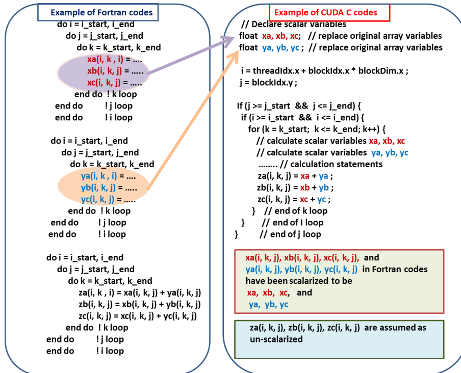
Figure 7. Illustration of scalarizing temporary arrays by scalar variable in order to recalculate values in the local memory rather than transferring them from global memory to local memory. In this illustration, xa , xb , xc , ya , yb , yc are assumed to be scalarizable, but za , zb , zc are assumed to be un-scalarizable. Note that the regular mathematical array syntax is used to express the arrays.
