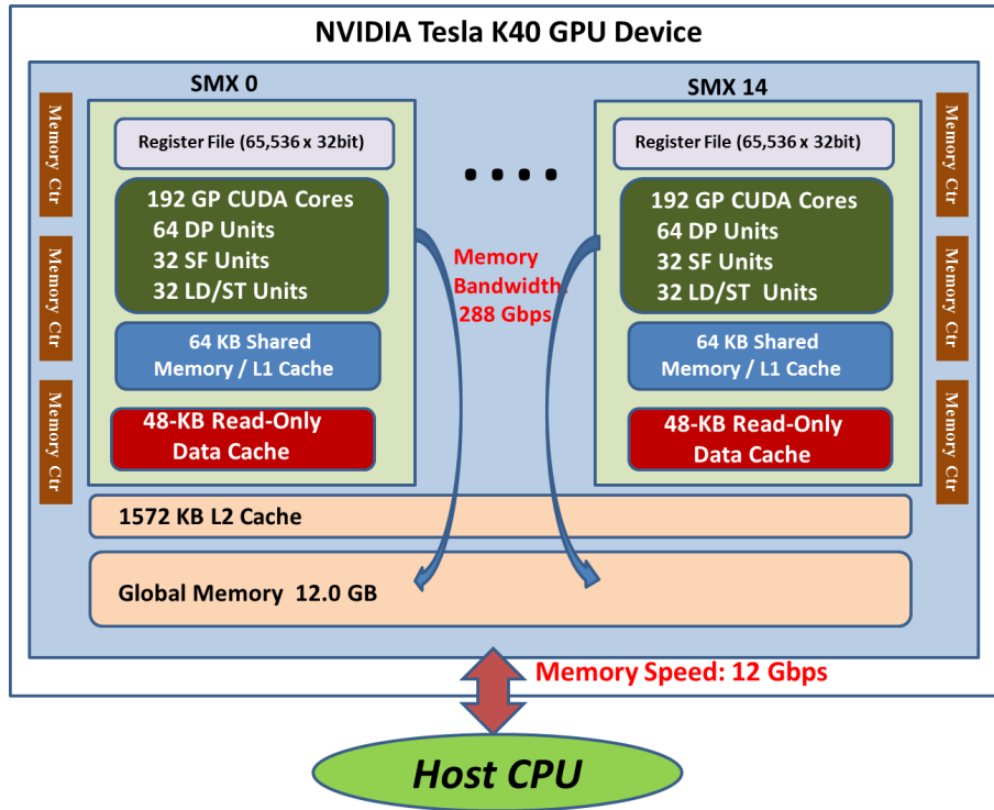
Figure 2. Schematic diagram of hardware specification of one NVIDIA Tesla K40 GPU employed in our study.
