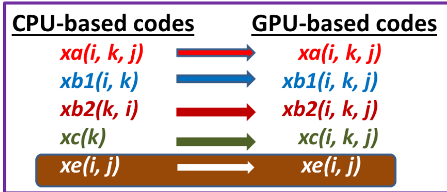
Figure 6. Illustration for re-arranging arrays in CPU-based implementation to 3-D and 2-D arrays in GPU-based implementation, where regular mathematical array syntax is used to express the arrays.
