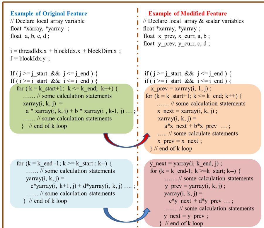
Figure 8. Illustration for how to release height dependence in order to reduce the access time to global memory for those temporary arrays which have dependence among the (k - 1) th, k th, and (k + 1) th components. The left (right) figure is the original (modified) CUDA program.
