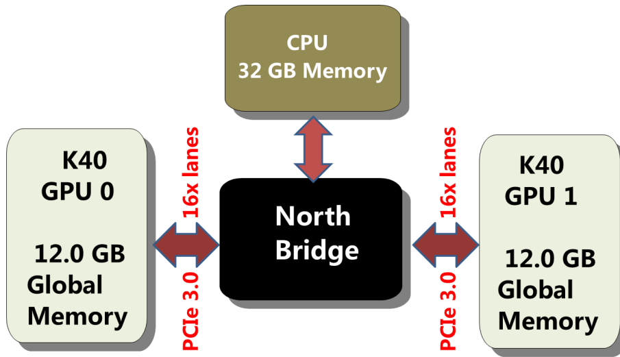
Figure 13. Schematic diagram of our multi-GPU setup.
