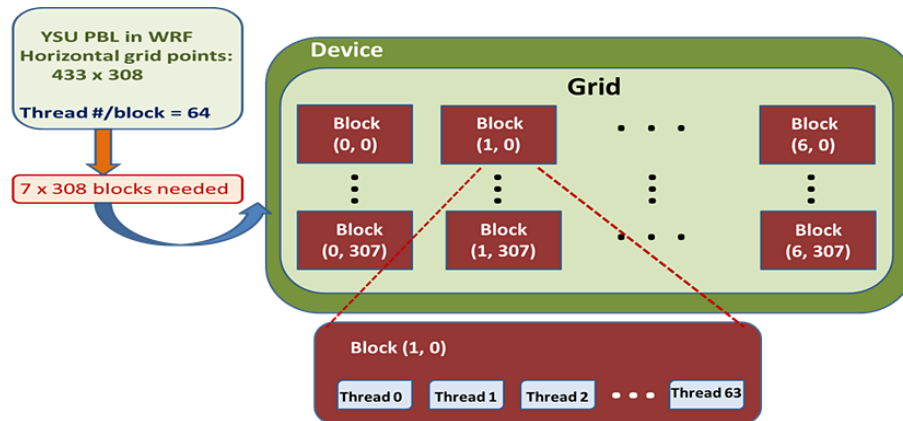
Figure 3. Three-level thread hierarchy of a device for one GPU utilized in our study: threads, thread block, and grids of block.
