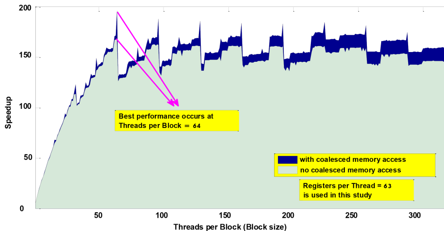
Figure 9. Speedup vs. threads per block (block size) for optimized GPU-based YSU PBL scheme.
