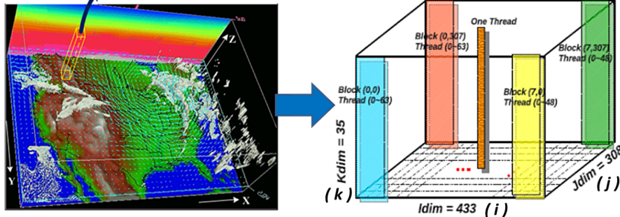
Figure 4. Mapping of the CONUS domain onto one GPU thread-block-grid domain, where the size of the CONUS domain is 433 \times 308 horizontal grid point with 35 vertical levels.
