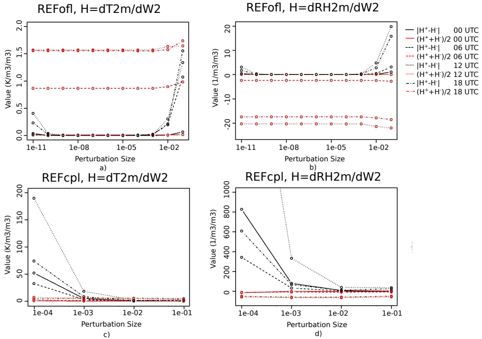
Figure 8. Comparison of the optimal perturbation size for the offline (top) and coupled (bottom) approach. |\mathbf{H}^+ - \mathbf{H}^-| (black) and \mathbf{H}^+ + \mathbf{H}^-/2 (red) for different perturbation sizes on 2 July 2010 at 00:00, 06:00, 12:00 and 18:00 UTC averaged over the whole domain with \mathbf{H} = \delta T_{2m}/\delta W_2 (left) and \mathbf{H} = \delta RH_{2m}/\delta W_2 (right).
