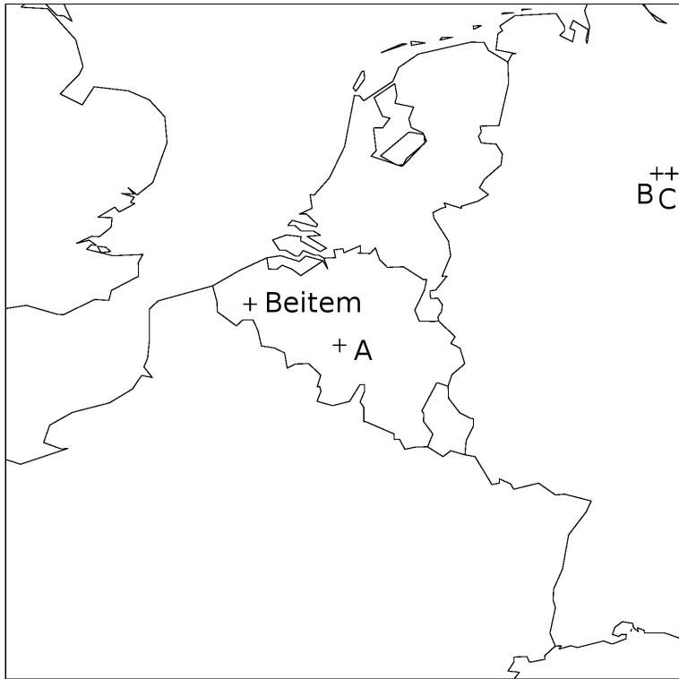
Figure 2. The operational 4 km ALARO-Belgium domain. The indicated locations will be used in the following sections. Beitem: 50.905^{\circ} N, 3.123^{\circ} E (Belgium). Location A: 50.534^{\circ} N, 4.497^{\circ} E (Belgium). Location B: 52.092^{\circ} N, 9.488^{\circ} E (Germany). Location C: 52.082^{\circ} N, 9.722^{\circ} E (Germany)
