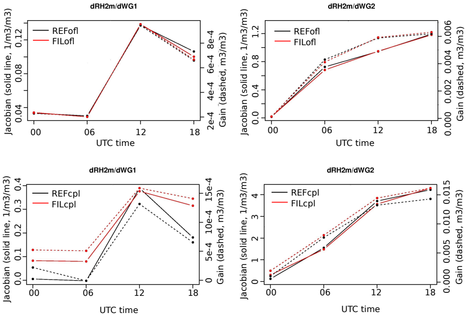
Figure 10. Jacobian and gain values for the \delta RH_{2m}/\delta W_s and \delta RH_{2m}/\delta W_2 averaged over the whole domain on 2 July 2010 for REF Fofl , FIL Fofl , REF cpl and FIL cpl for 00:00, 06:00, 12:00 and 18:00 UTC. The solid lines represent the Jacobian values (values on the left vertical axis), the dashed lines represent the gain values (values on the right vertical axis).
