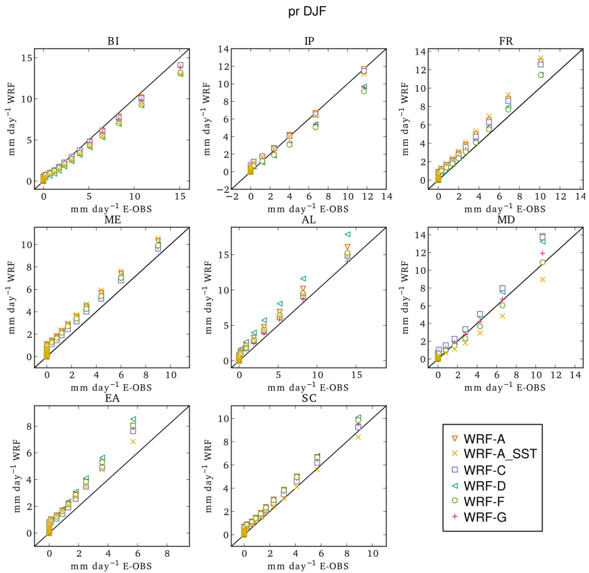
2 Figure S2b Quantile-quantile plots computed for the European subregions for mean winter 3 1990-2008 precipitation.
