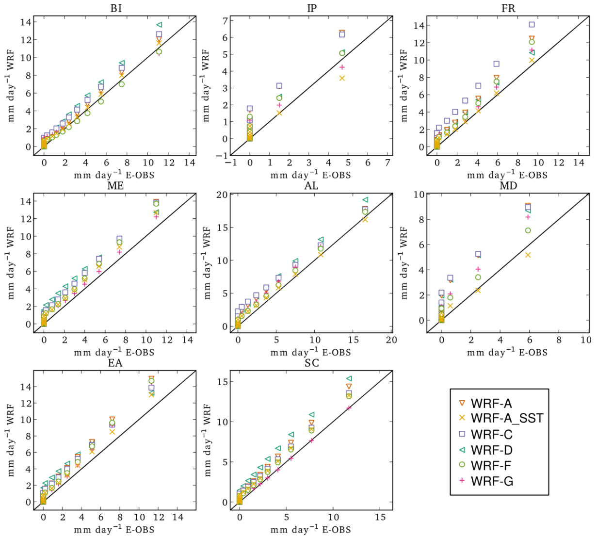
2 Figure S2a Quantile-quantile plots computed for the European subregions for mean summer 3 1900-2008 precipitation.
