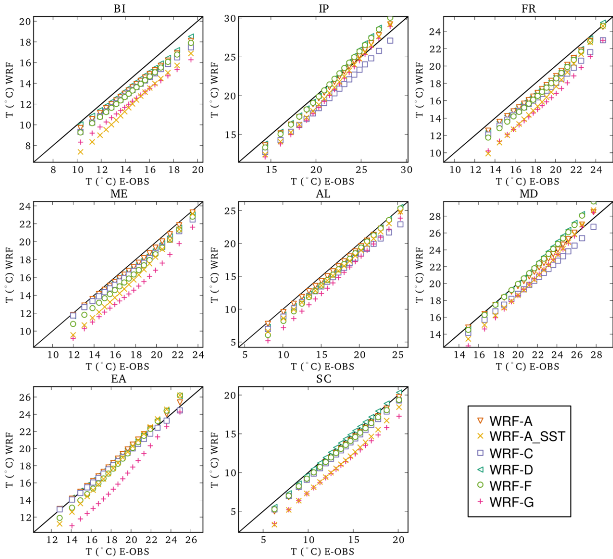
1 2 Figure S1a Quantile-quantile plots computed for the European subregions for mean summer 3 1990-2008 temperature.
