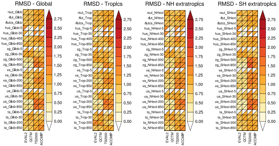
Figure 5. Root-mean square difference of the chosen basic climate parameters over the global domain, the tropics, and the NH and SH extratropics (from left to right, respectively). Columns and rows of each panel represent the EMAC simulations and the given diagnostics (see Table 3), respectively. Where an alternative dataset is available, the diagram boxes are split in two parts, showing the model performance compared to the primary (lower triangle) and alternative (upper triangle) dataset. Where no observations are available, the triangles are marked white.
