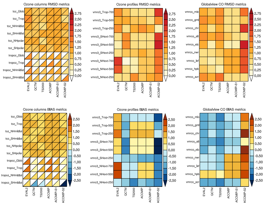
Figure 11. Root-mean square difference (top) and overall mean bias (bottom) for total and tropospheric column ozone (left), ozone profiles (middle) and surface CO diagnostics (right). Columns and rows of each panel represent the EMAC simulations (including the sensitivity experiments) and the given diagnostics (see Table 3), respectively. Where an alternative dataset is available, the diagram boxes are split in two parts, showing the model performance compared to the primary (lower triangle) and alternative (upper triangle) dataset. Where no observations are available, the triangles are marked white.
