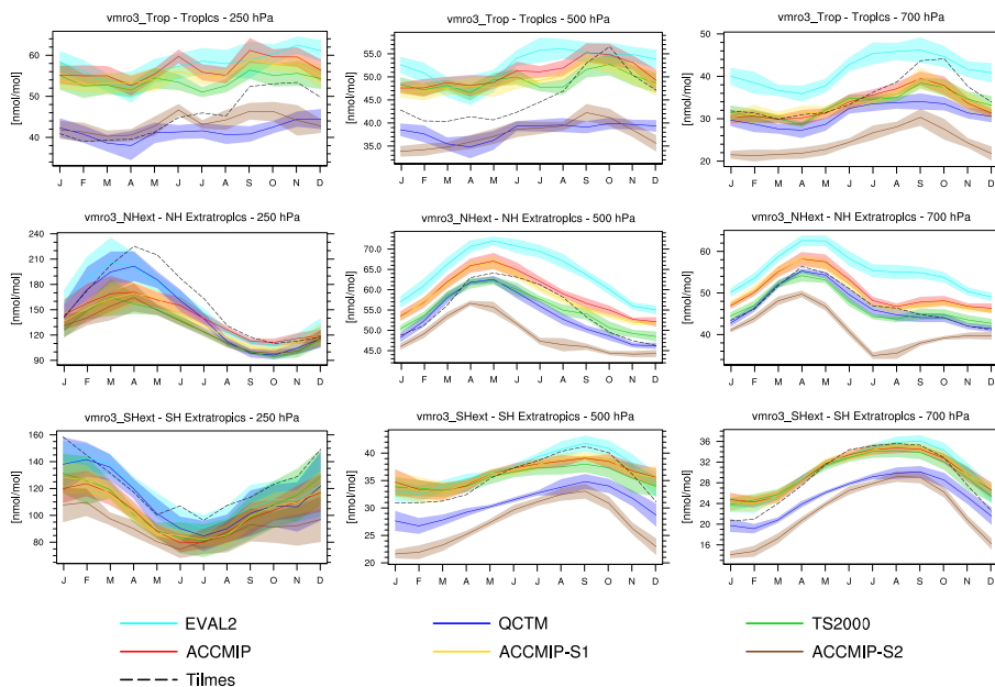
Figure 15. Annual cycle of ozone climatology in three regions (tropics, NH and SH extratropics) at three pressure levels (250, 500 and 700 hPa) for the EMAC simulations compared with ozonesonde data by Tilmes et al. (2012). Model and observational data are grouped into four latitude bands and sampled at three, with the models sampled at the ozonesonde locations before averaging together. The tropical region is represented by 9 stations, NH and SH extratropics by 22 and 5 stations, respectively (see Fig. S14). The shaded areas indicate the \pm 1\sigma interannual variability (for EMAC only).
