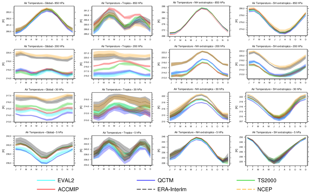
Figure 1. Annual cycle of temperature climatology at 850, 200, 30 and 5 hPa averaged globally, over the tropics (20° S–20° N), NH extratropics (20–90° N) and SH extratropics (20–90° S) for the EMAC simulations, in comparison to ERA-Interim and NCEP/NCAR reanalysis data. Shaded areas indicate the \pm 1\sigma interannual variability.
