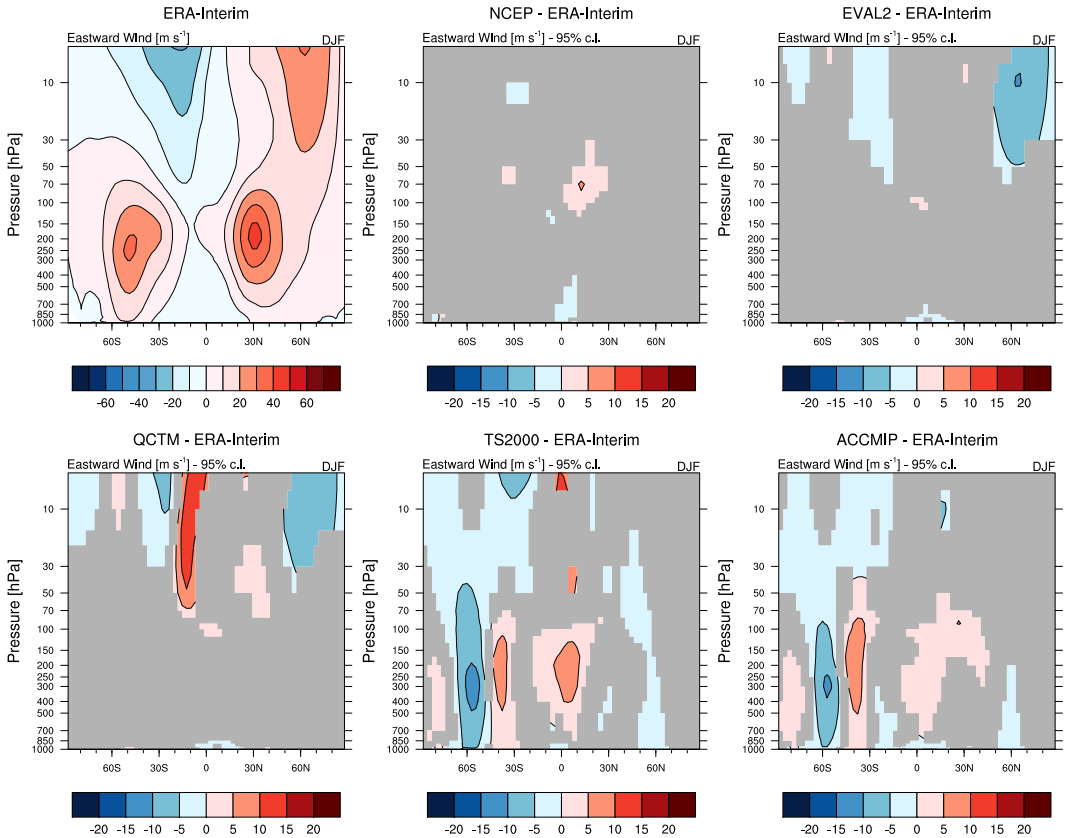
Figure 9. As in Fig. 2, for seasonal (DJF) mean of zonally averaged eastward wind profile.
