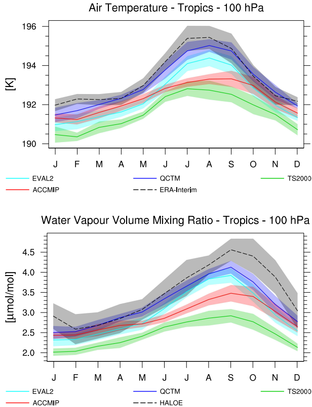
Figure 4. Annual cycle of temperature (top) and water vapour (bottom) climatology at 100 hPa averaged over the tropics ( 20^{\circ} N– 20^{\circ} S) for the EMAC simulations, in comparison to ERA-Interim re-analysis and HALOE data, respectively. Shaded areas indicate the \pm 1\sigma interannual variability.
