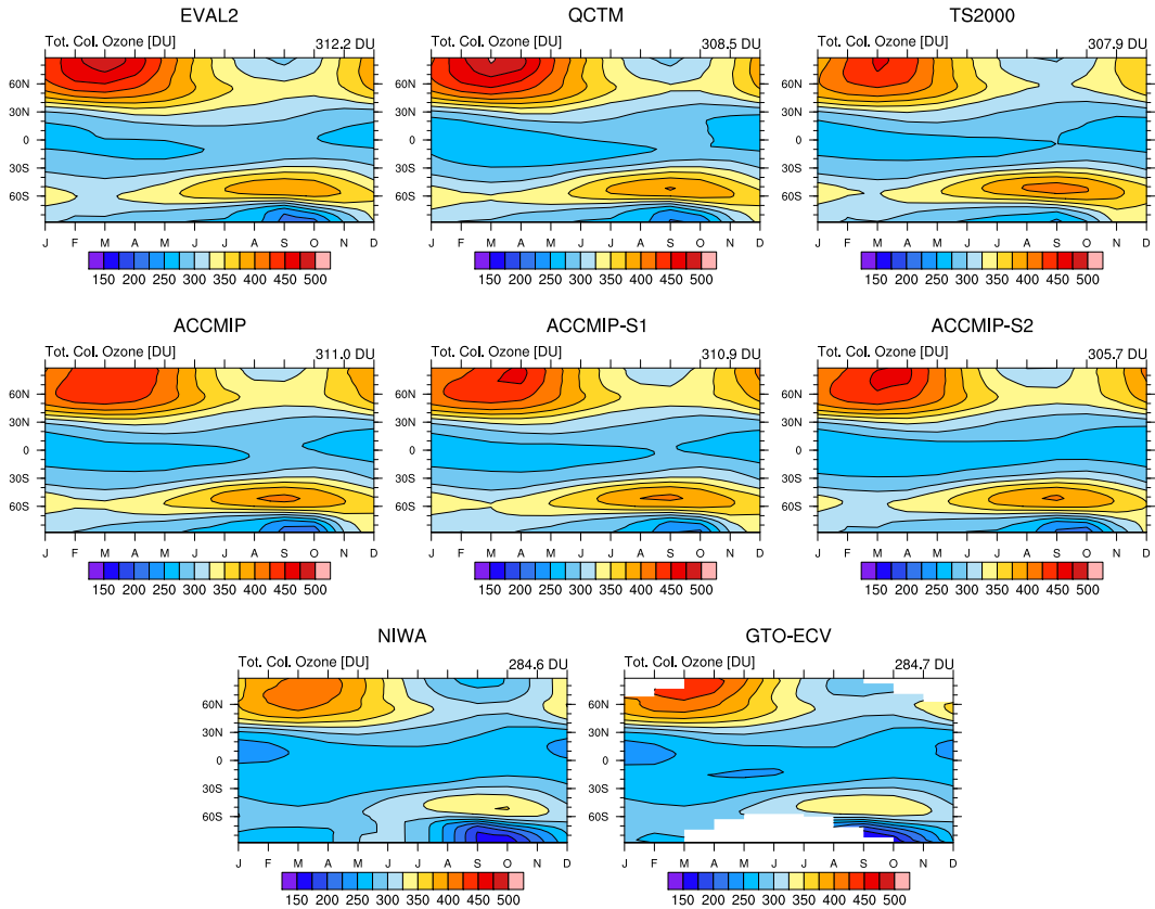
Figure 10. Total column ozone climatology for the EMAC simulations compared to the NIWA combined total column ozone database and GTO-ECV data. The values on top of each panel show the global (area-weighted) average, calculated after regridding the data to the horizontal grid of the model and ignoring the grid cells without available observational data in the GTO-ECV data.
