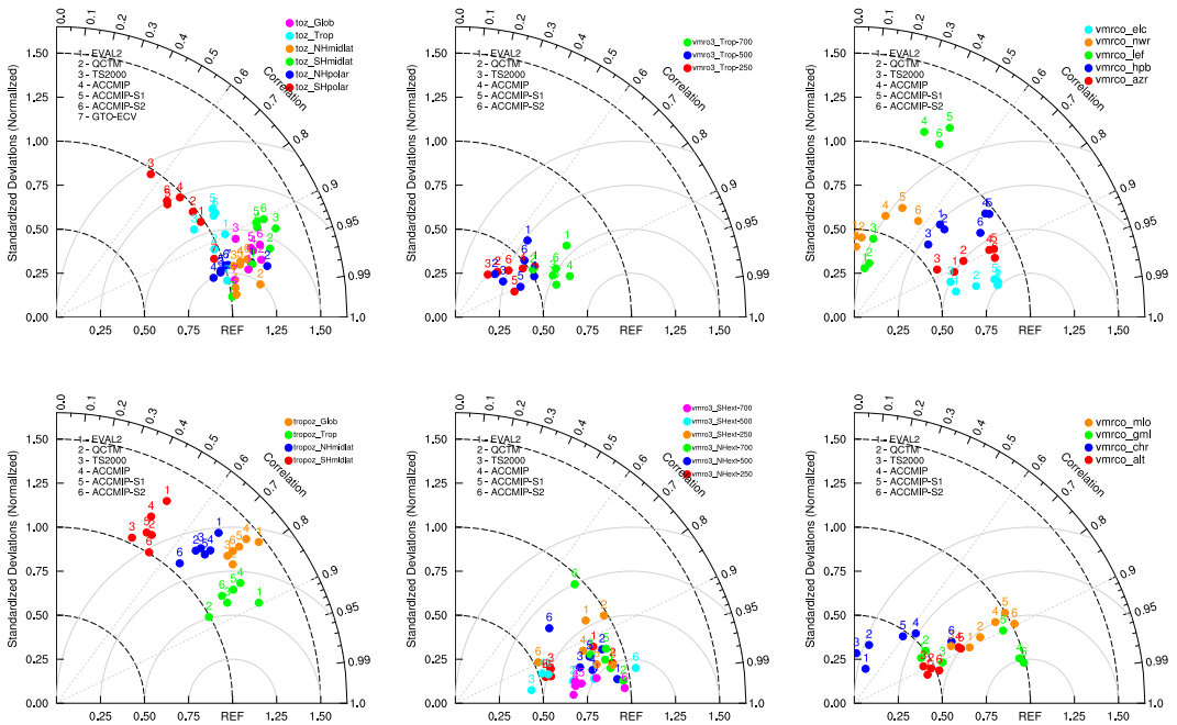
Figure 12. Taylor diagrams for total and tropospheric column ozone (left), ozone profiles (middle) and surface CO diagnostics (right).
