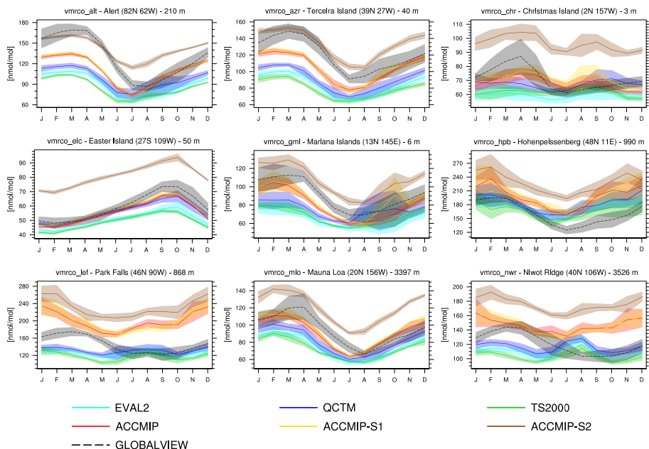
Figure 18. Annual cycle of CO surface concentration climatology for the EMAC simulations and NOAA GLOBALVIEW data, at nine different stations world wide. The shaded areas indicate the \pm 1\sigma interannual variability.
