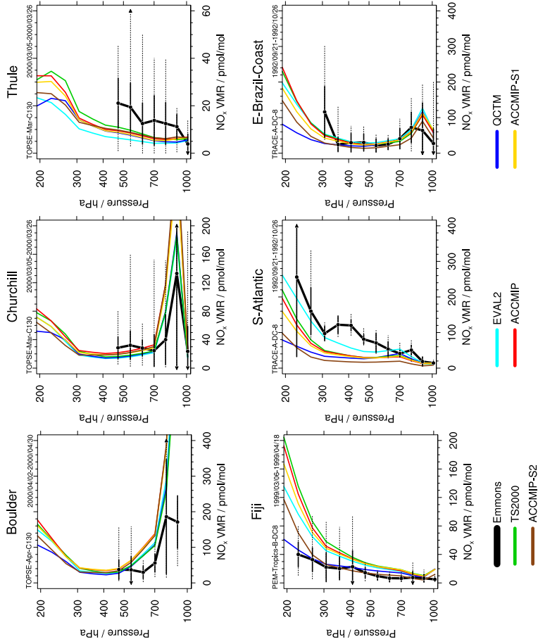
Figure 17. Similar to Fig. 16, for NO x .
