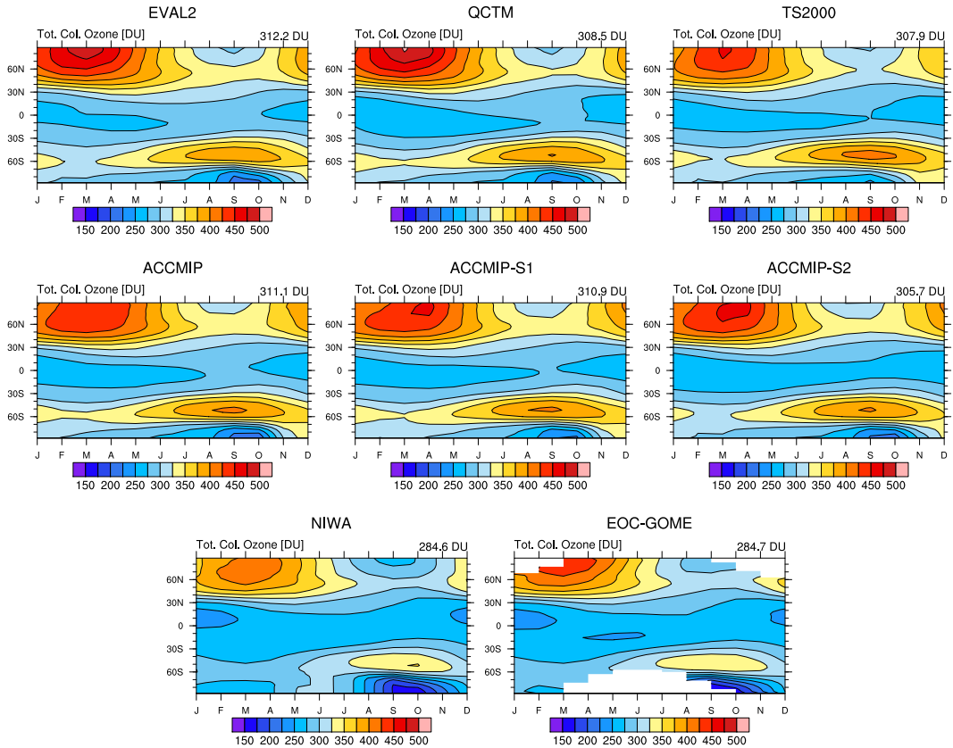
Figure 10. Total column ozone climatology for the EMAC simulations compared to the NIWA combined total column ozone database and GOME data. The values on top of each panel show the global (area-weighted) average, calculated after regridding the data to the horizontal grid of the model and ignoring the grid cells without available observational data in the GOME dataset.
