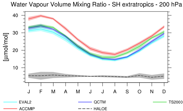
Figure 3. Annual cycle of water vapour climatology at 200 hPa averaged over the SH extratropics ( 20\text{--}90^\circ\text{S} ) for the EMAC simulations in comparison to HALOE data. Shaded area indicates the \pm 1\sigma interannual variability.
