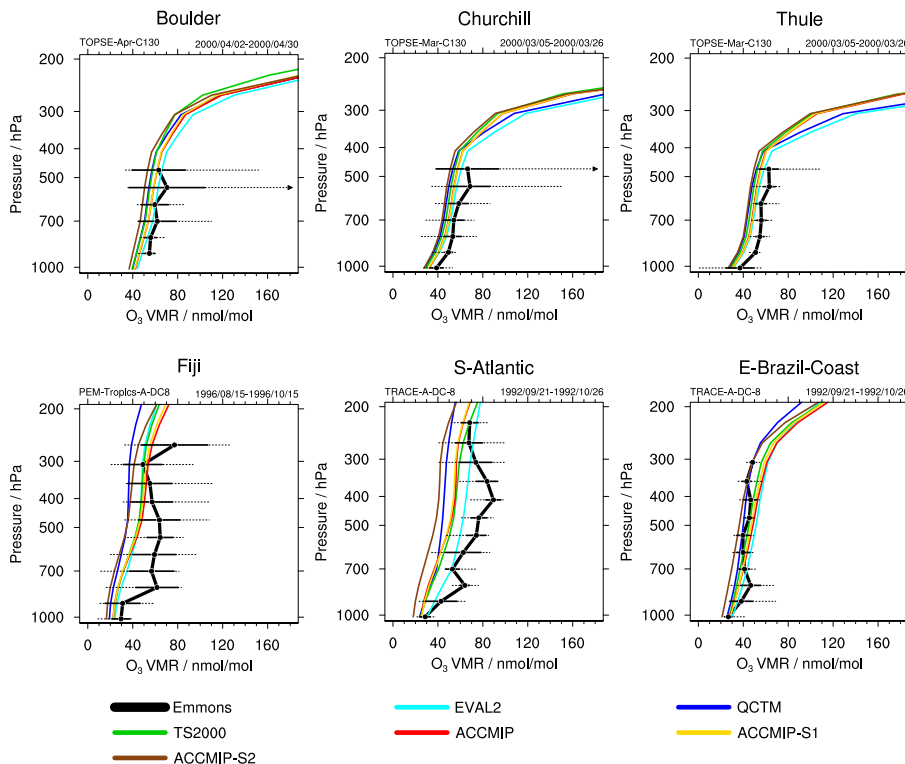
Figure 16. Ozone vertical profile climatology from selected aircraft campaign observations by Emmons et al. (2000) and corresponding simulated values by the EMAC simulations. Profiles represent mean values. The EMAC simulations are averaged over the same regions and time of year as the observations, but for different years. Solid whiskers indicate \pm 1 standard deviation and dotted whiskers show minimum and maximum, both for the observational data.
