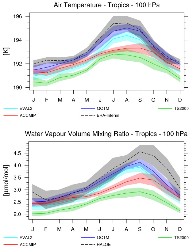
Figure 4. Annual cycle of temperature (top) and water vapour (bottom) climatology at 100 hPa averaged over the tropics (20° N–20° S) for the EMAC simulations, in comparison to ERA-Interim re-analysis and HALOE data, respectively. Shaded areas indicate the \pm 1\sigma interannual variability.
