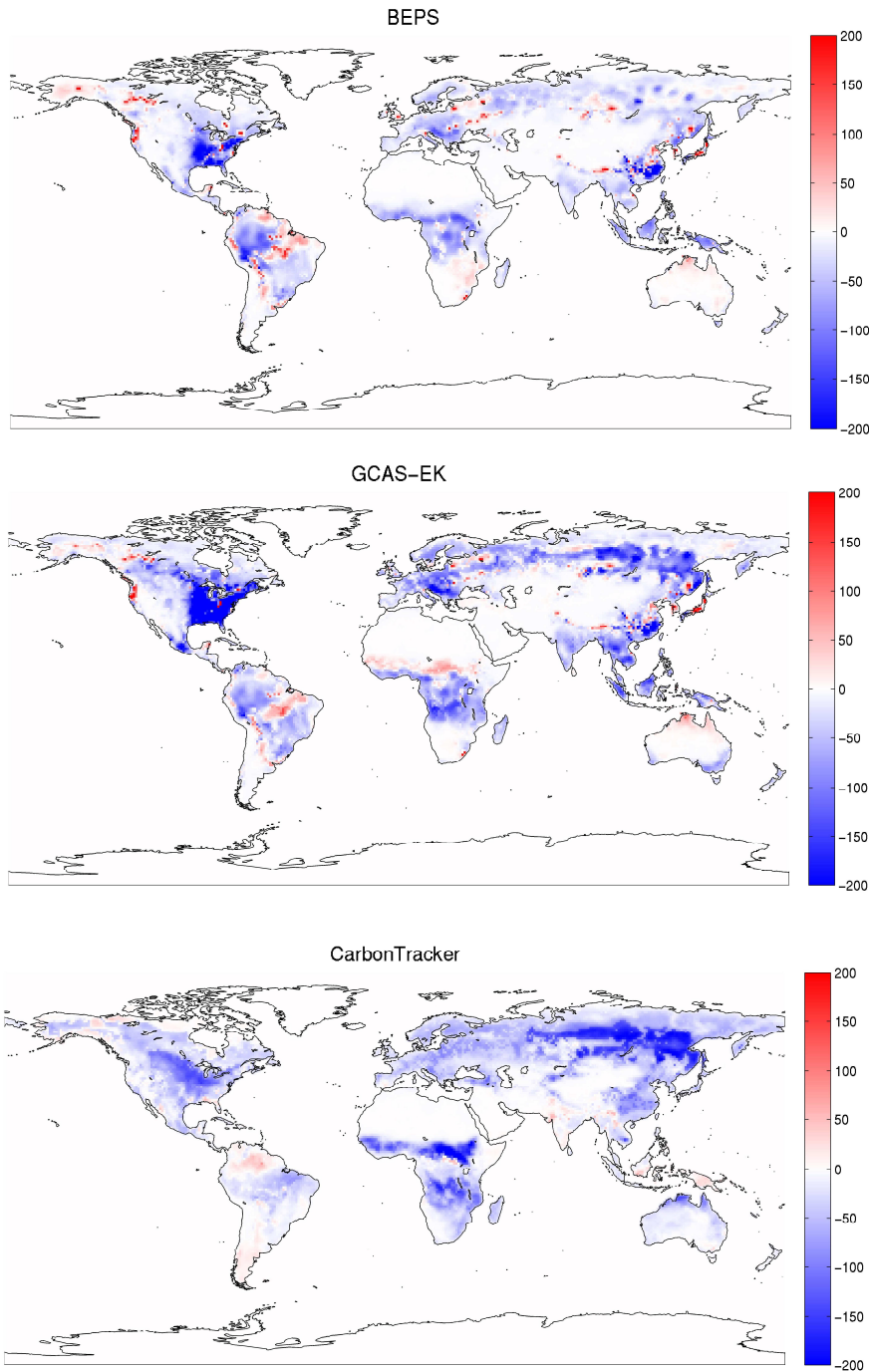
Figure 7. Global carbon budget (gC m -2 ) distributions on multiyear average from 2002 to 2008: prior carbon fluxes simulated by BEPS; assimilated carbon fluxes by GCAS-EK; CarbonTracker 2011 estimated carbon fluxes.
