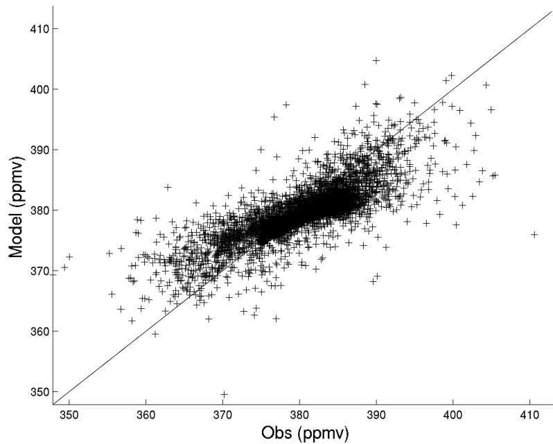
1 2 Figure 6. Comparisons between real observations and simulated concentrations 3 by control runs: top) control run forcing by prior carbon fluxes; bottom) control 4 run forcing by assimilated carbon fluxes by GCAS-EK. Both simulations start 5 from Jan 1,2002 and all simulated concentrations at observation locations and 6 times in 2005 are compared here.
