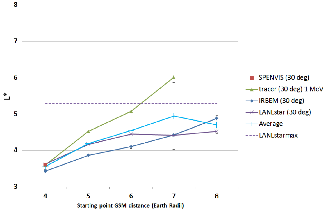
Figure 7. Calculations of L^* as a function of initial distance (in R_E ) at 0 MLT, for an initial pitch angle of 30 degrees during disturbed solar wind conditions. Error bars represent the standard deviation between results from the various models.
