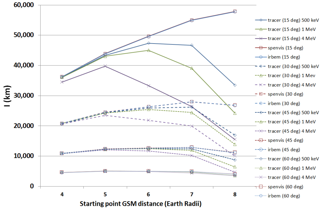
Figure 2. Calculations of I as a function of initial distance (in R_E ) at 0 MLT, for pitch angles of 15, 30, 45 and 60 degrees and quiet solar wind conditions.
