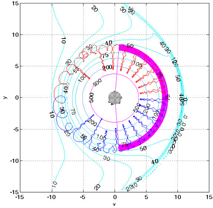
Figure 11. The Lorenz trace of the forward (blue) and backwards (red) propagating particle is plotted. The region where I is constant according to Fig. 10 is shown in magenta. The contours of constant magnetic field strength are also plotted.
