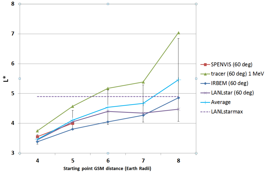
Figure 8. Calculations of L^* as a function of initial distance (in R_E ) at 0 MLT, for an initial pitch angle of 60 degrees during disturbed solar wind conditions. Error bars represent the standard deviation between results from the various models.
