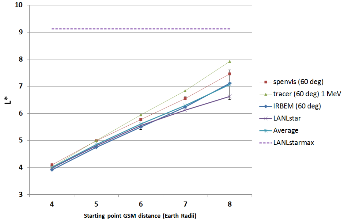
Figure 5. Calculations of L^* as a function of initial distance (in R_E ) at 0 MLT, for an initial pitch angle of 60 degrees during quiet solar wind conditions. Error bars represent the standard deviation between results from the various models.
