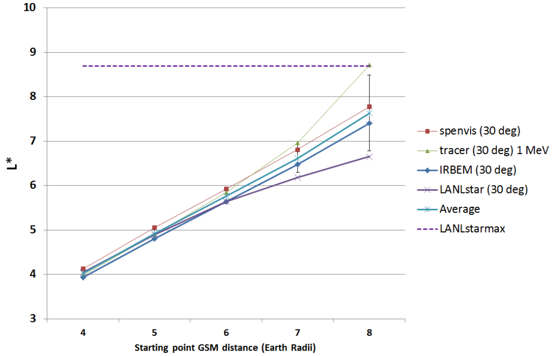
Figure 4. Calculations of L^* as a function of initial distance (in R_E ) at 0 MLT, for an initial pitch angle of 30 degrees during quiet solar wind conditions. Error bars represent the standard deviation between results from the various models.
