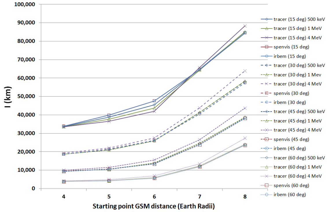
Figure 3. Calculations of I as a function of initial distance (in R_E ) at 12 MLT, for pitch angles of 15, 30, 45 and 60 degrees and disturbed solar wind conditions.
