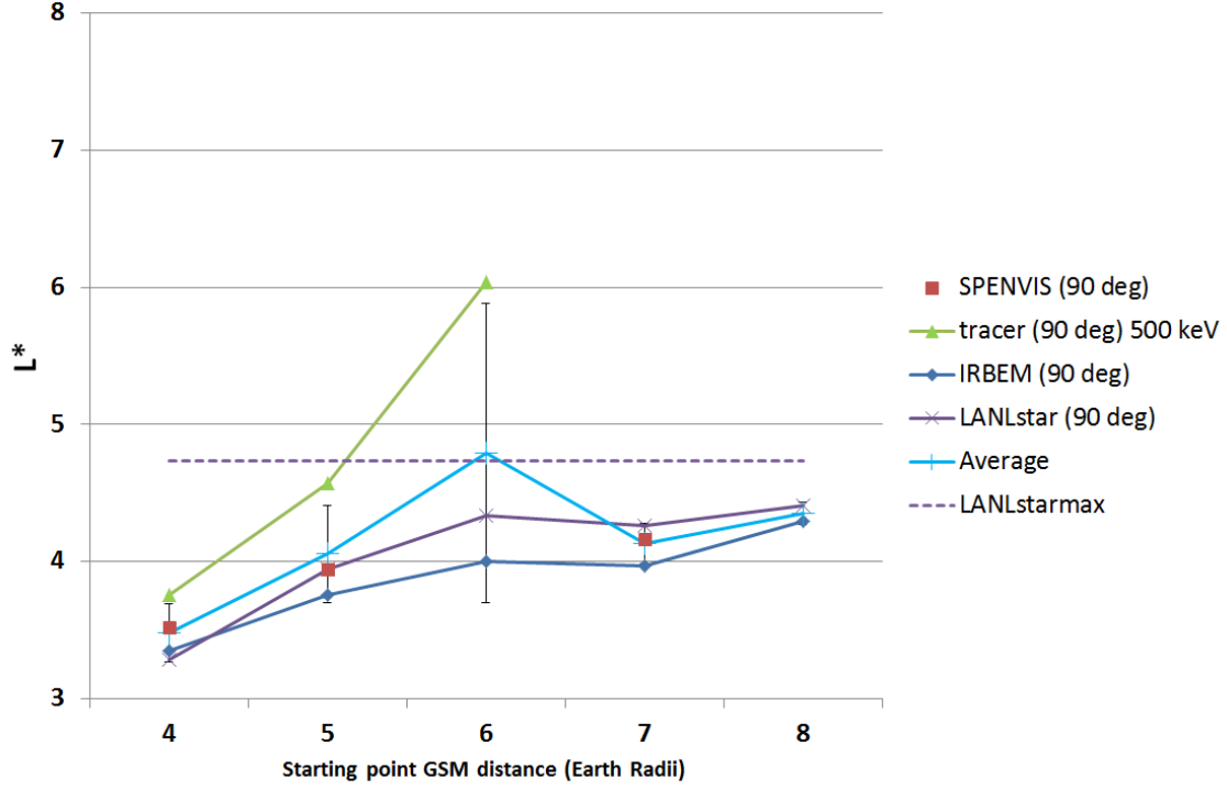
Figure 9. Calculations of L^* as a function of initial distance (in R_E ) at 0 MLT, for an initial pitch angle of 90 degrees during disturbed solar wind conditions. Error bars represent the standard deviation between results from the various models.
