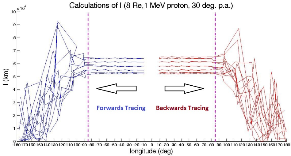
Figure 10. I as a function of the particle's azimuth angle for the case 1 MeV protons starting at GSM coordinates [8, 0, 0] (in R_E ) with initial pitch angles of 30 deg, and initial gyrophases of 0-330^\circ ( 30^\circ step). Particles propagating forward in time are shown in blue, while those propagating backwards are shown in red.
