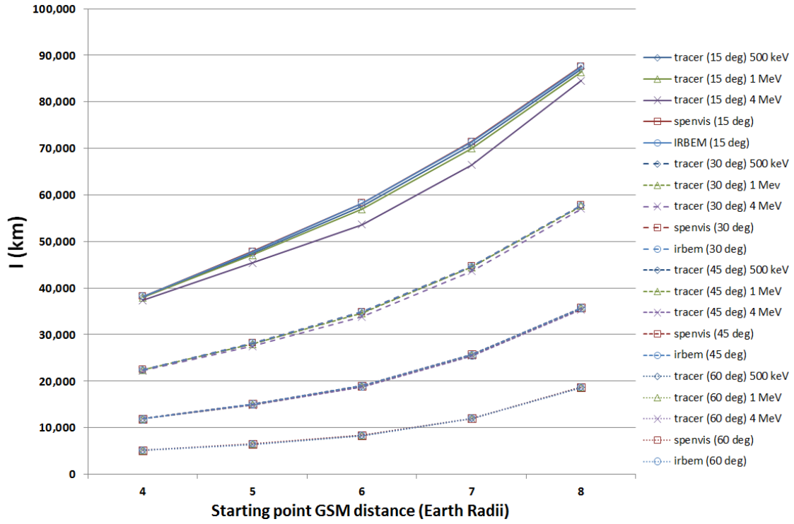
Figure 1. Calculations of I as a function of initial distance (in R_E ) at 12 MLT, for pitch angles of 15, 30, 45 and 60 degrees and quiet solar wind conditions.
