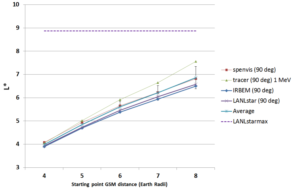
Figure 6. Calculations of L^* as a function of initial distance (in R_E ) at 0 MLT, for an initial pitch angle of 90 degrees during quiet solar wind conditions. Error bars represent the standard deviation between results from the various models.
