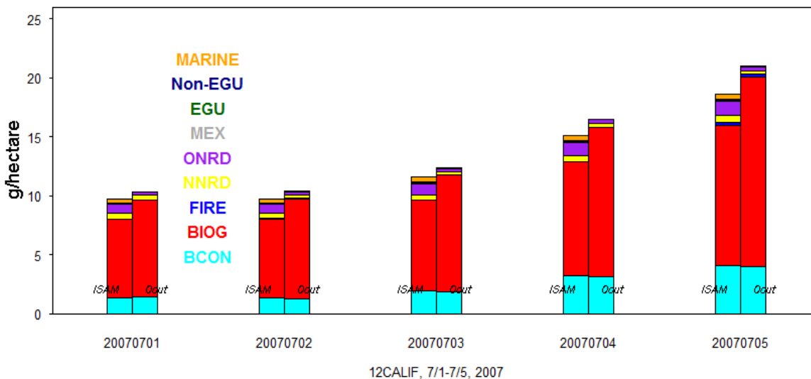
Supp Figure 11. Daily-total, domain-averaged VOC deposition (dry+wet), July 1-5, 2007. As in Fig. 6, for each day left column designates ISAM total, and right one the zero-out. The colors represent sector sources: marine (MARINE orange), non-electricity generation units (NON-EGU deep blue), electricity generation units (EGU green), Mexican point sources (MEX light grey), on-road mobile (ONRD purple), non-road mobile (NNRD yellow), wild fires (FIRE blue), BIOG3 vegetations (BIOG red), and boundary conditions (BCON cyan).
