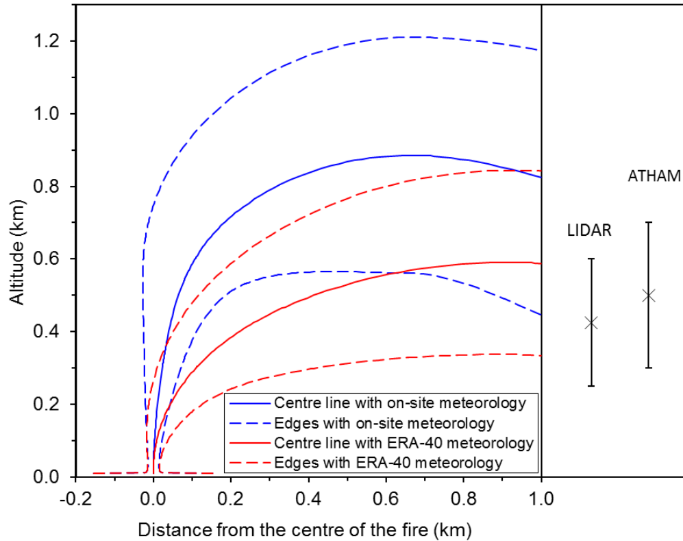
Fig. 3. Simulated altitude of the centre line, and the lower and upper edges of the plume for the Quinault prescribed burn as a function of the downwind distance. The results are shown both for using (i) the meteorological measurements made on site (blue solid and dashed lines, denoted by “on-site meteorology”) and (ii) the re-analysis of the meteorological observations (red solid and dashed lines, denoted by “ERA 40 meteorology”). The vertical ranges of the previous results obtained using on-site LIDAR measurements (“LIDAR”; Trentmann et al., 2002) and computations using the ATHAM model (Trentmann et al., 2002) have also been presented.
