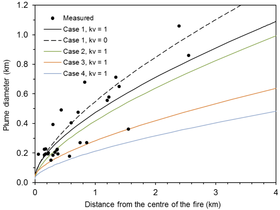
Fig. 7. The measured and predicted plume diameters against downwind distance from the centre of the fire, for cases 1-4. The data of measurements are presented as black dots, and predictions as solid and dotted lines.
