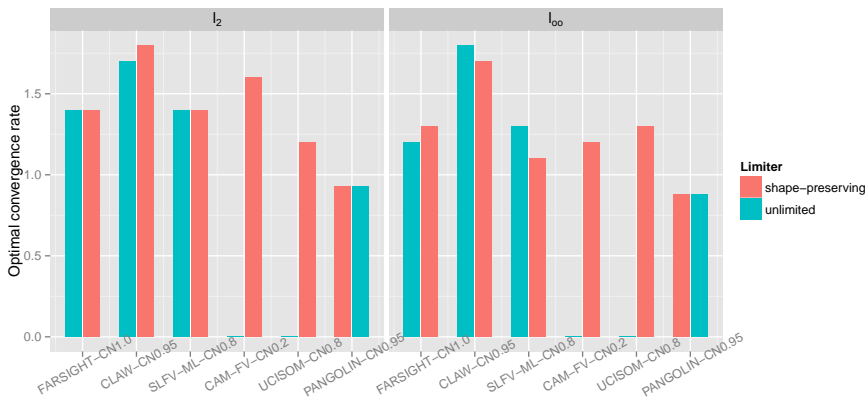
Figure 9. Optimal order of convergence computed by a least-square regression on data from Fig. 8. Some models did not offer data without shape-preserving limiters (CAM-FV, UCISOM).
