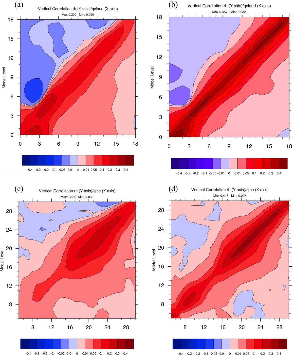
3 Figure 14. (a) Raw vertical cross-correlations between cloud mixing ratio ( q_{cloud} ) and relative 4 humidity (rh), (b) filtered vertical cross-correlations between q_{cloud} and rh, (c) raw vertical 5 cross-correlations between ice mixing ratio ( q_{ice} ) and rh, (d) filtered vertical cross-correlations 6 between q_{ice} and rh. Taking into account the perturbations coming from the transition of a
