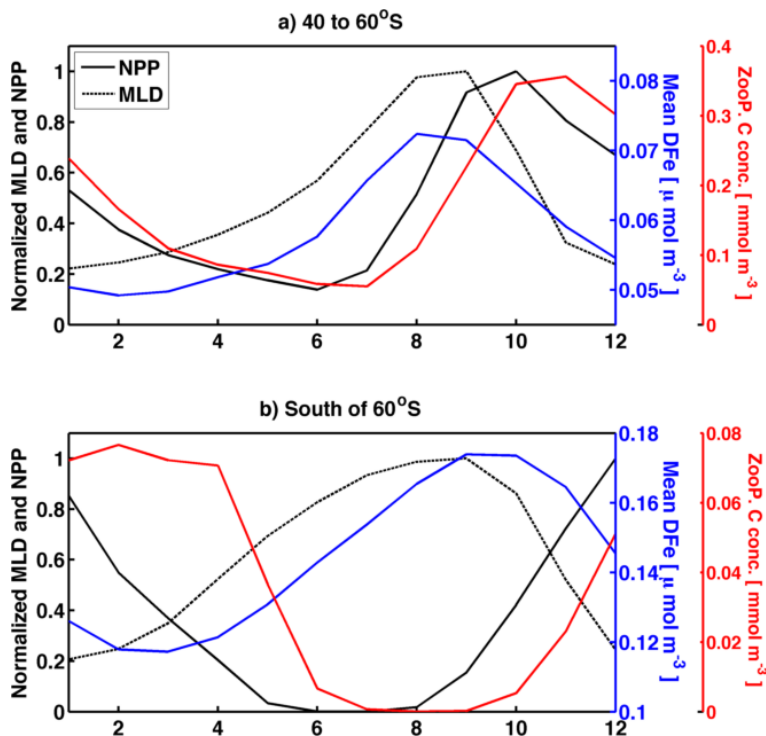
Fig. 20. Seasonal change in the modelled NPP, MLD, DFe and zooplankton concentration for: (a) the Southern Ocean from 40 to 60° S and (b) south of 60° S. DFe and zooplankton concentrations are averaged over the top 100 m of the ocean. NPP and MLD are normalized by the maximum of the monthly values.
