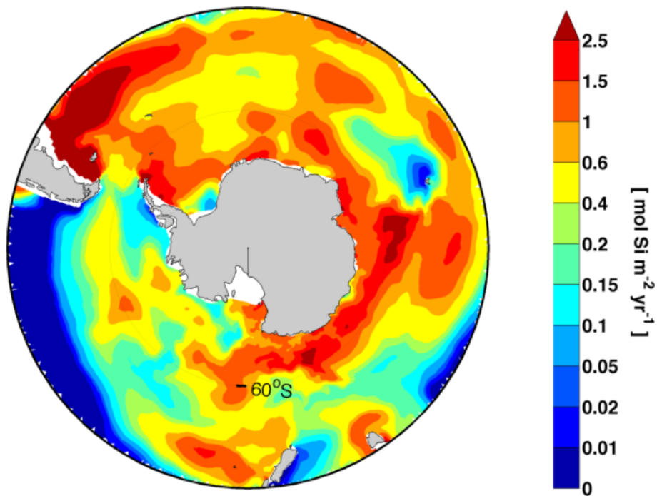
Fig. 17. Modelled export of opal across 100 m depth plotted to the scale used by Moore et al. (2004).
