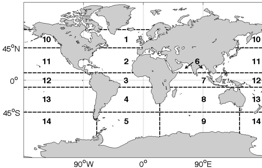
Fig. 3. Map of the ocean regions used to examine the model results on basin scale.
