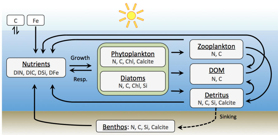
Fig. 2. The pathways in the biogeochemical model REcoM2.
