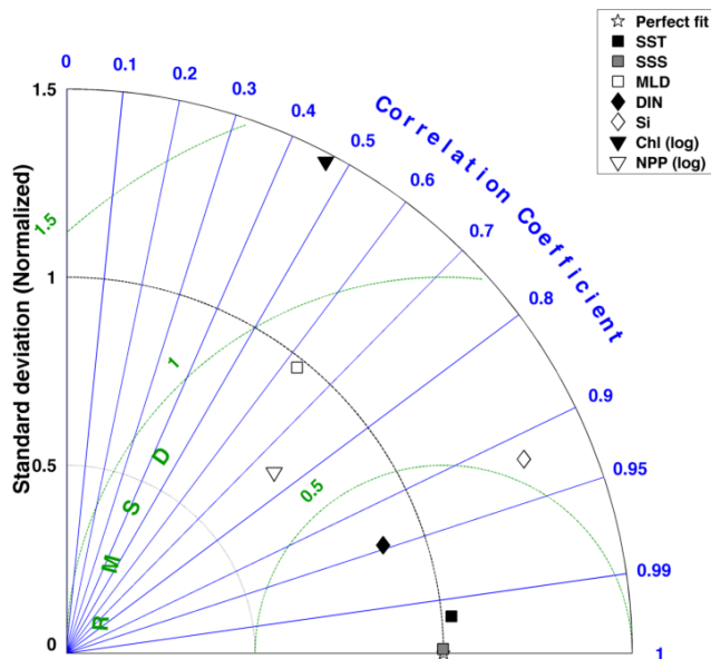
Fig. 15. Taylor diagram for the Southern Ocean south of 50° S showing correlation, normalized standard deviation and the normalized root mean square error between the spatial distribution of the model results and observed data sets, weighted by area. All values are surface values, except the mixed layer depth and the NPP, which is vertically integrated. The fields have been linearly interpolated to a 1° by 1° grid, similar to the World Ocean Atlas. Dividing with the observed standard deviation has normalized the model standard deviation and root mean square error.
