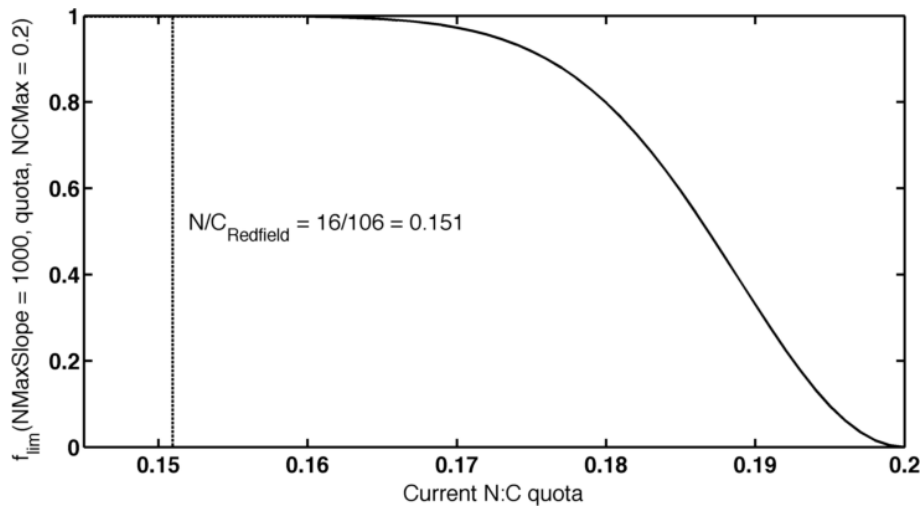
Fig. 22. Change in limiter function f_{\text{lim}}^{N:C_{\text{max}}} with N : C quota.
