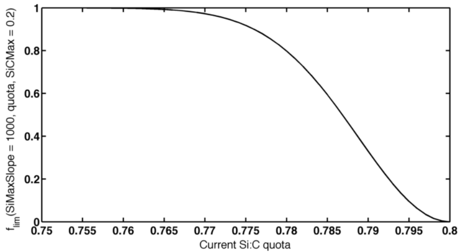
Fig. 24. Change in limiter function with Si : C quota.
