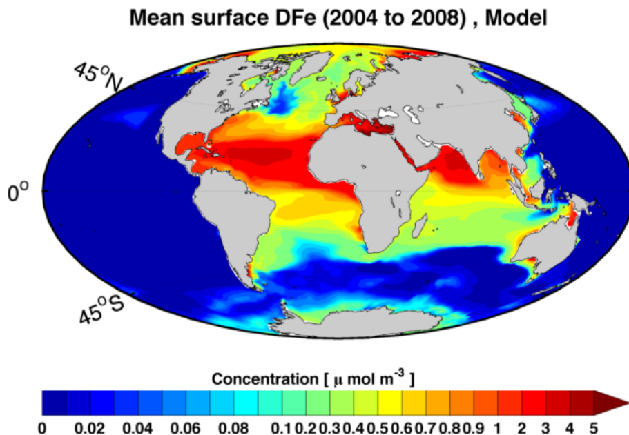
Fig. 9. Spatial distribution of the mean surface concentration of dissolved iron. Plotted to the scale used by Schneider et al. (2008).
