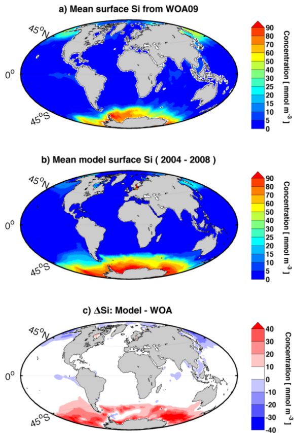
Fig. 8. Spatial distribution of mean surface concentration of dissolved inorganic silicon. (a) Observed (Garcia et al., 2010) (b) Modelled. (c) Residual: Modelled – observed.
