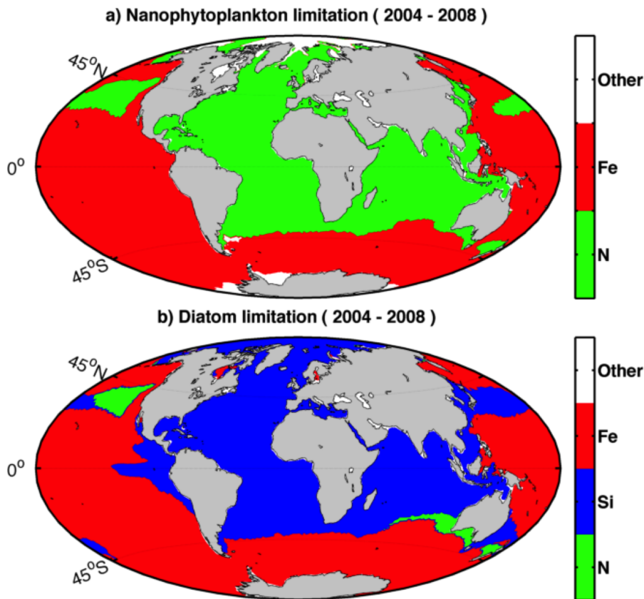
Fig. 10. Following the example of Schneider et al. (2008), the spatial distribution of the annually mean limiting nutrients in the model's surface water has been calculated. (a) Nanophytoplankton (Fe = 56.6 %, DIN = 40.1 % of total area). (b) Diatoms (Fe = 53.6 %, DIN = 2.5 % and DSi = 43.8 % of total area).
