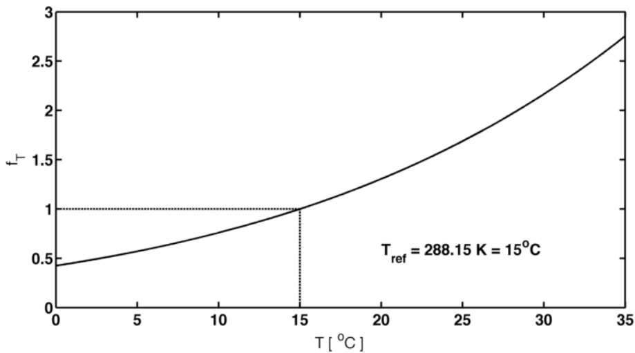
Fig. 21. The Arrhenius function plotted with the parameters used in REcoM2.
