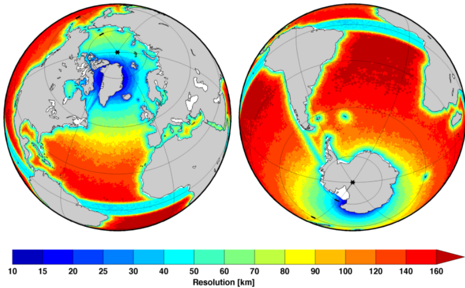
Fig. 1. Horizontal resolution of FESOM's unstructured grid.
