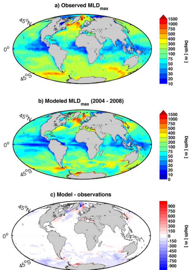
Fig. 5. Mean spatial distribution of the MLD_{max} over the years 2004 to 2008. (a) Observation based (de Boyer Montegut et al., 2004). (b) Modelled. (c) Residual: Modelled – observation based.
