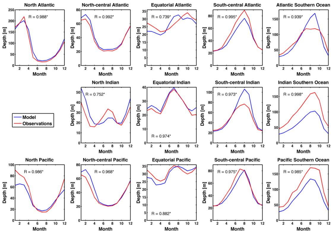
Fig. 6. Mean MLD over the year in the ocean basins depicted in Fig. 3. The correlation coefficient is written in each plot, and the statistically significant correlations ( p values < 0.05 ) are marked with *.
