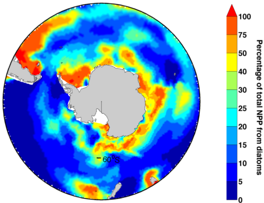
Fig. 16. Contribution of diatoms to NPP in the model.
