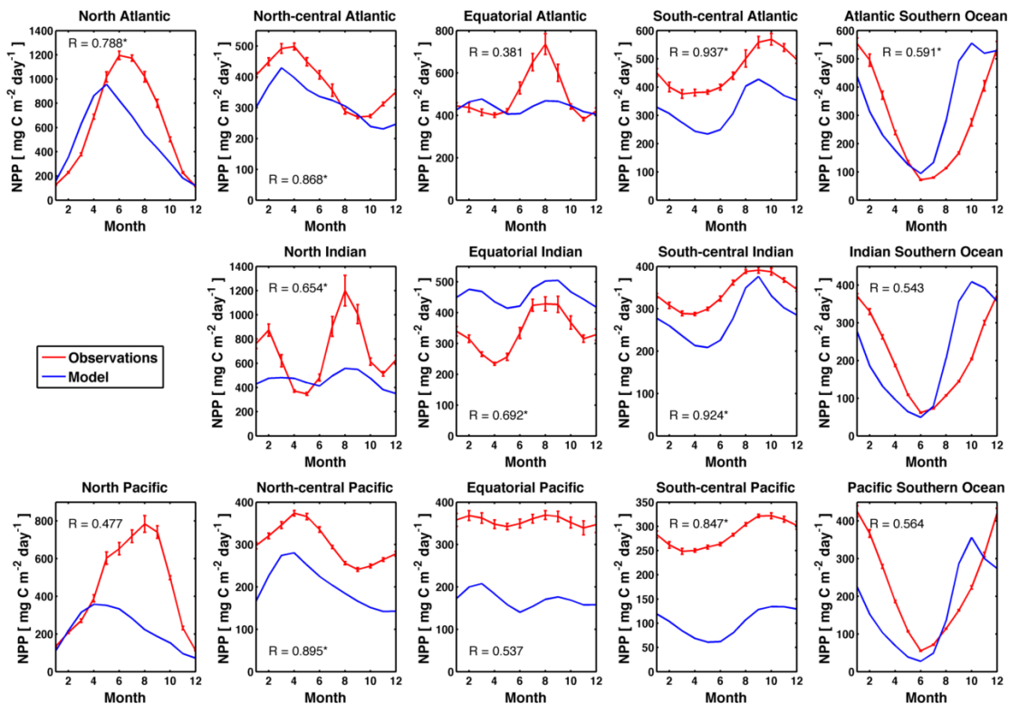
Fig. 13. Mean NPP over the year in the ocean basins depicted in Fig. 3. The correlation coefficient is written in each plot, and the statistically significant correlations ( p values < 0.05) are marked with *.
