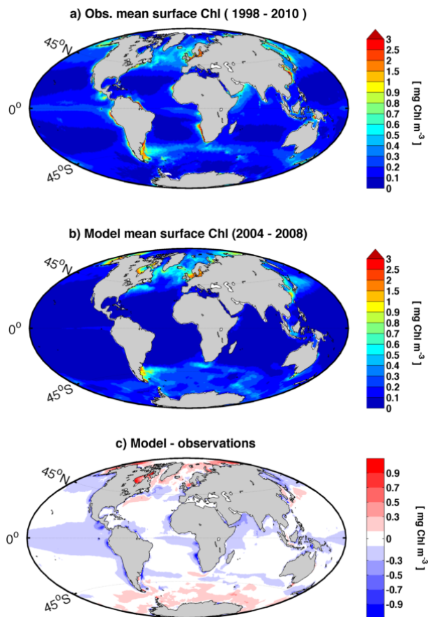
Fig. 11. Spatial distribution of mean surface concentrations of chlorophyll a plotted to the scale used by Schneider et al. (2008). (a) satellite-based estimate ( www.globcolour.info ). (b) Modelled. (c) Residual: Modelled – satellite-based estimate.
