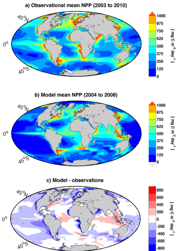
Fig. 12. Mean spatial distribution of vertically integrated net primary production plotted to the scale used by Schneider et al. (2008). (a) Satellite-based estimate (SeaWiFS and Behrenfeld and Falkowski, 1997). (b) Model. (c) Residual: Modelled – satellite-based estimate.
