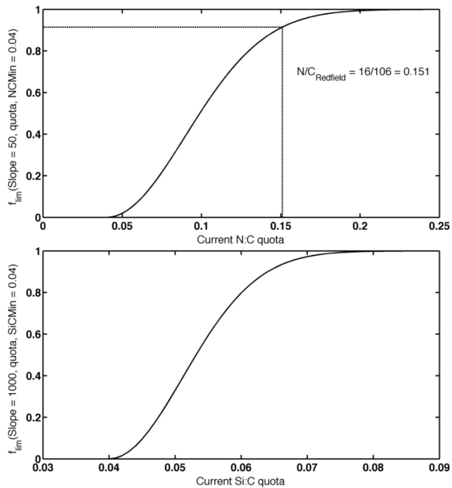
Fig. 23. Change in the limiter function f_{\lim}^{N:C^{\min}} with N:C quota.
