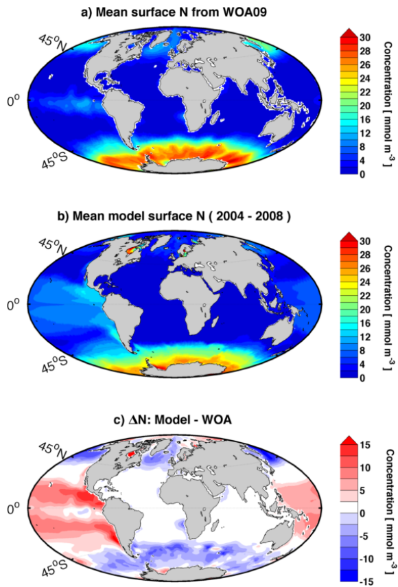
Fig. 7. Spatial distribution of mean surface concentration of dissolved inorganic nitrogen. (a) Observed (Garcia et al., 2010) (b) Modelled. (c) Residual: Modelled – observed.
