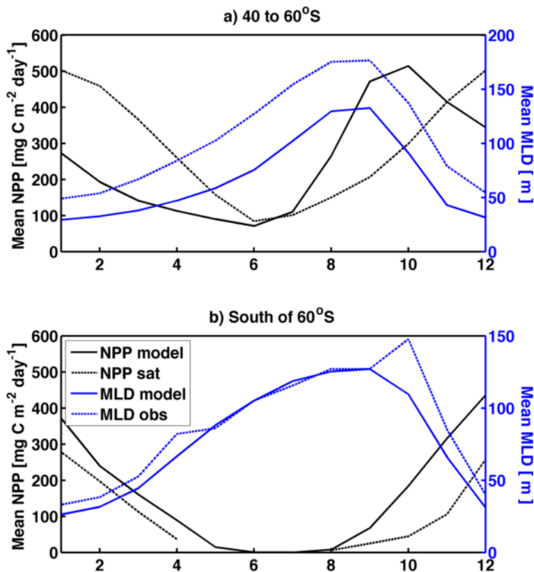
Fig. 19. Seasonal change in mean modelled and observed NPP (SeaWIFS and Behrenfeld and Falkowski, 1997) and MLD (de Boyer Montegut et al., 2004) for: (a) the Southern Ocean from 40 to 60° S and (b) south of 60° S.
