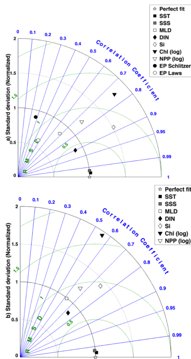
Fig. 4. Taylor diagrams (Taylor, 2001) showing correlation, normalized standard deviation and the normalized root mean square error between values of the model results and observations (Table 1), weighted by area. (a) Spatial distribution. (b) Spatial-seasonal distribution. All values are surface values, except the mixed layer depth and the vertically integrated NPP. (a) Uses the yearly mean calculated over 2004 to 2008 and (b) uses the monthly means of the same years. All fields have been interpolated to a 1^\circ by 1^\circ grid, using linear interpolation.
